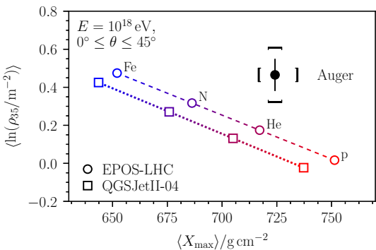
(b) E = 10^{18} \text{ eV}
