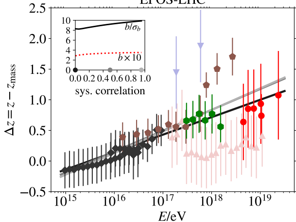
EPOS-LHC
