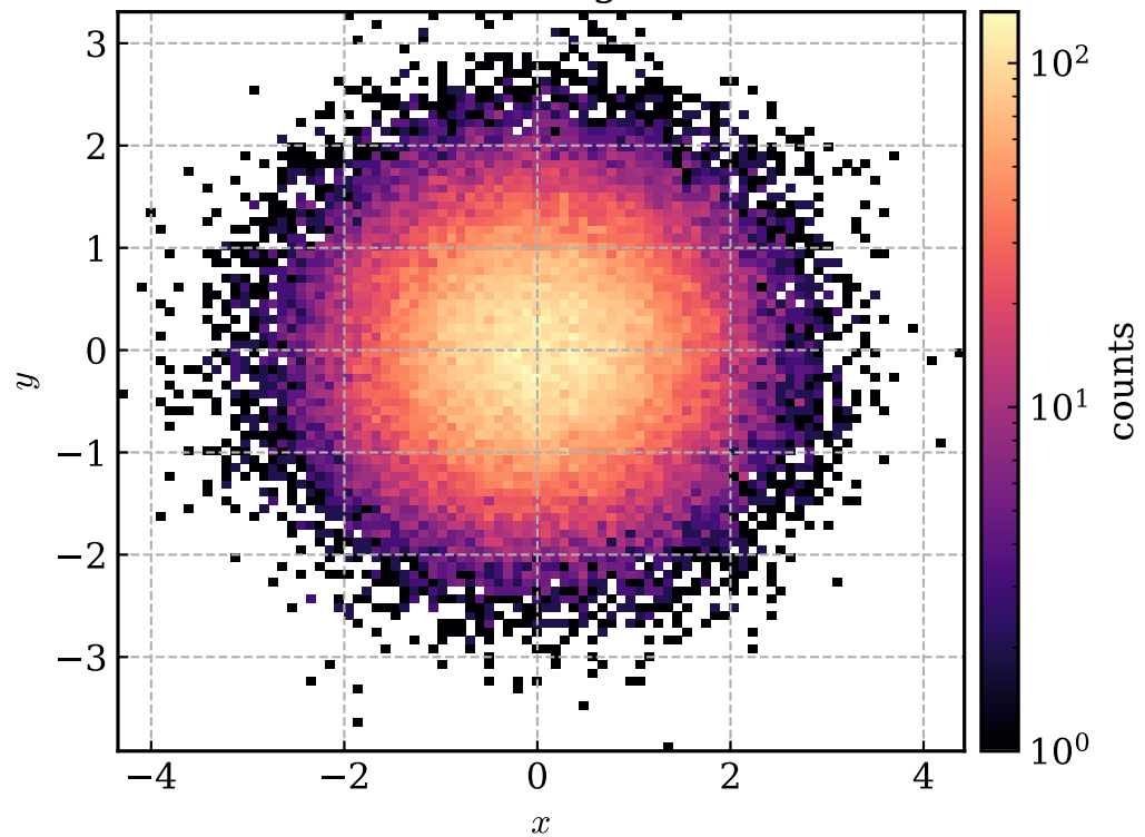
hist2d + LogNorm
