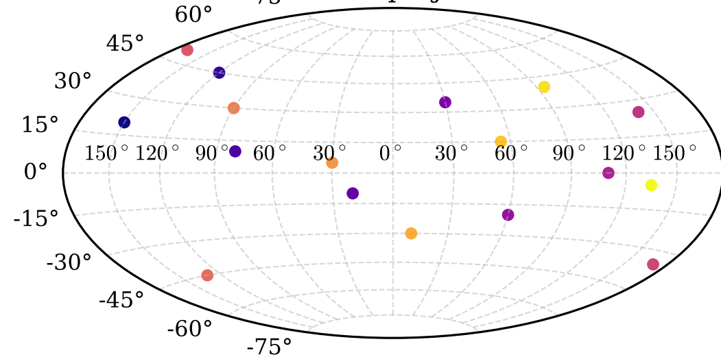
Hammer projection
