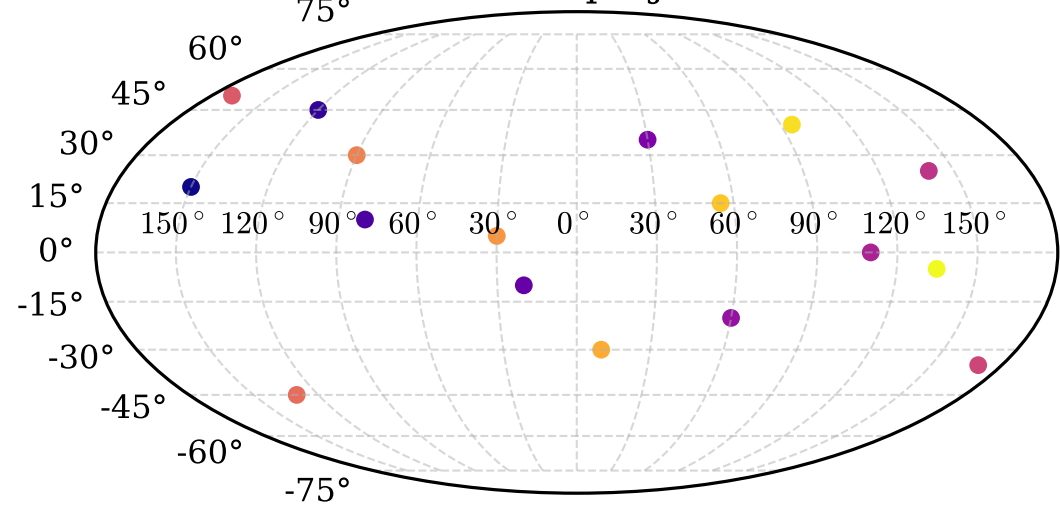
Mollweide projection
