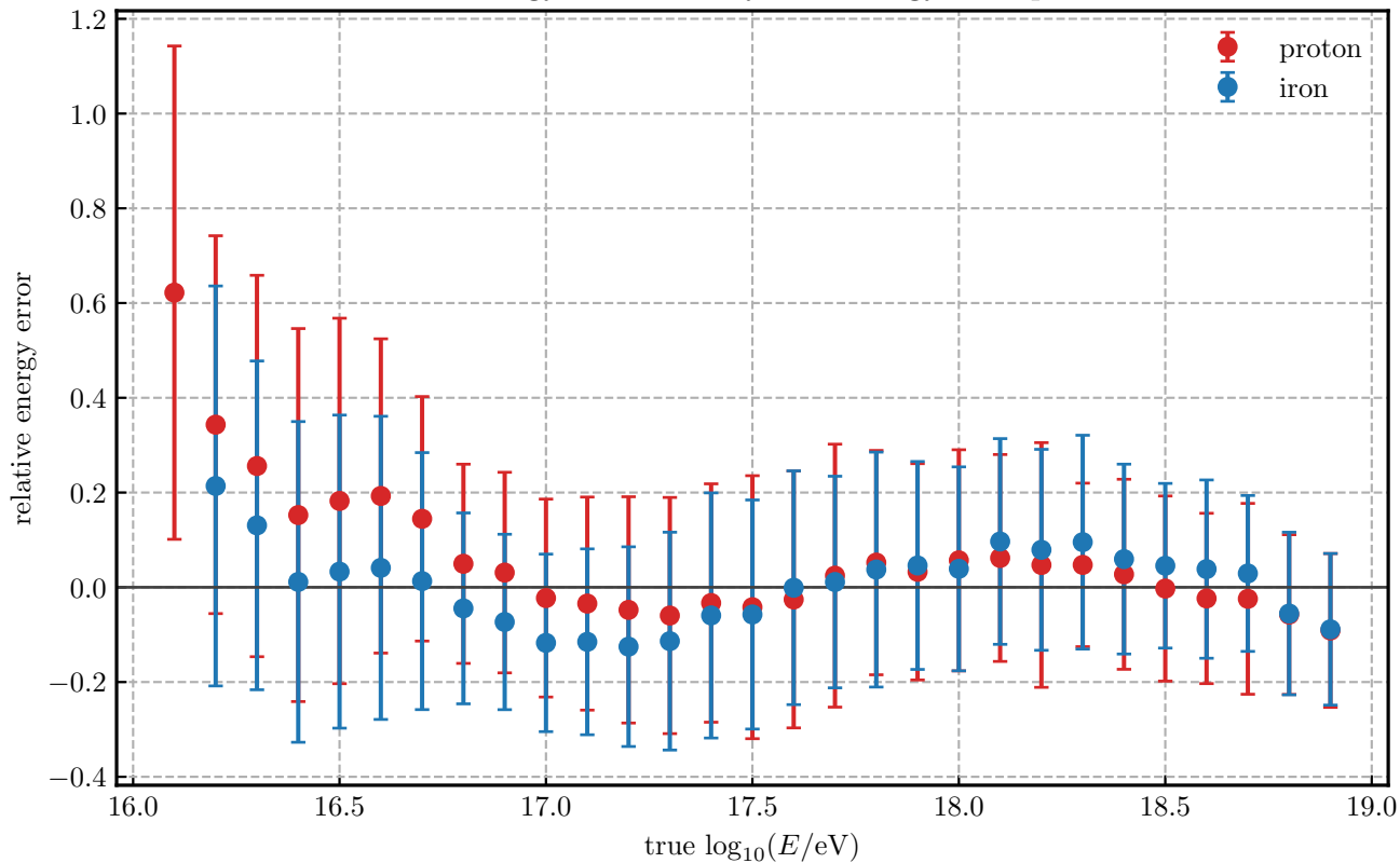
test: energy resolution by true energy and species
