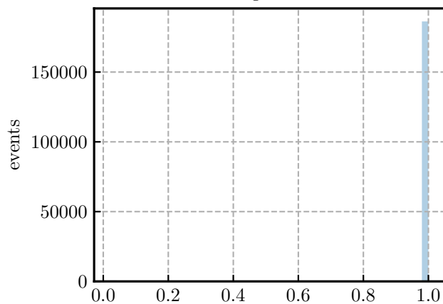
ising_causal
