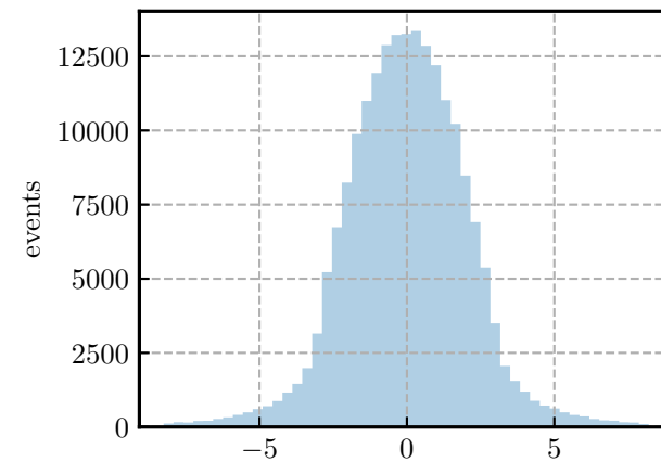
ising_causal_excess_usec
