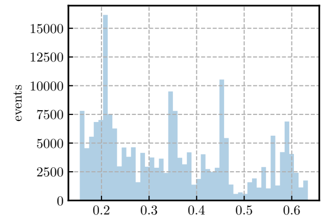
ising_spatial
