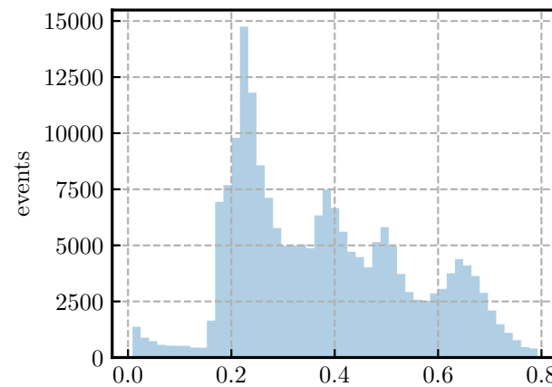
ising_weight_raw
