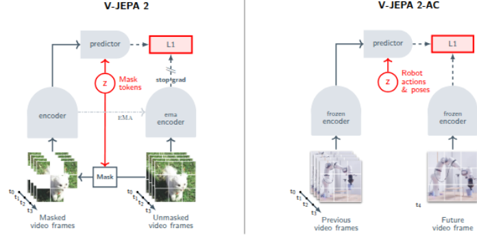
Figure 2.2 V-JEPA 2 multistage training (Assran et al., 2025). Left: self-supervised pre-training on internet-scale video with a mask-prediction objective in representation space. Right: the encoder is frozen and an action-conditioned predictor is learned on top; this thesis reuses only the frozen encoder.
