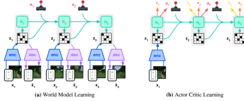
Figure 2.1 The DreamerV3 world model and actor-critic (Hafner et al., 2023). Observations are encoded into a compact latent state whose evolution a sequence model predicts from actions, and the actor and critic learn on trajectories imagined inside the model, conditioned on the agent's native action: the body-specific signal this thesis replaces.
