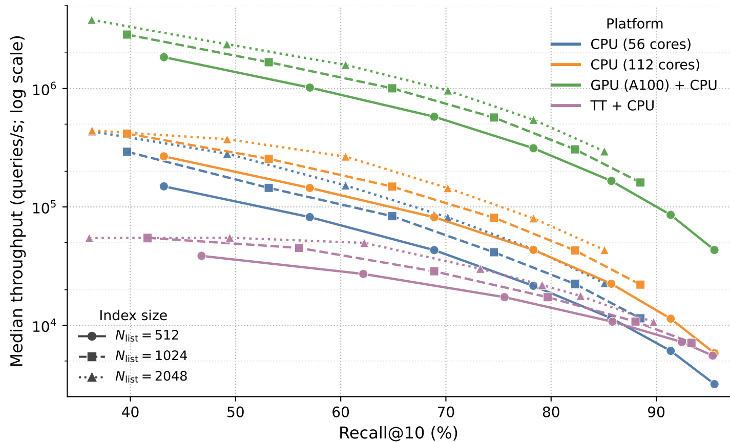
Throughput-recall trade-off
