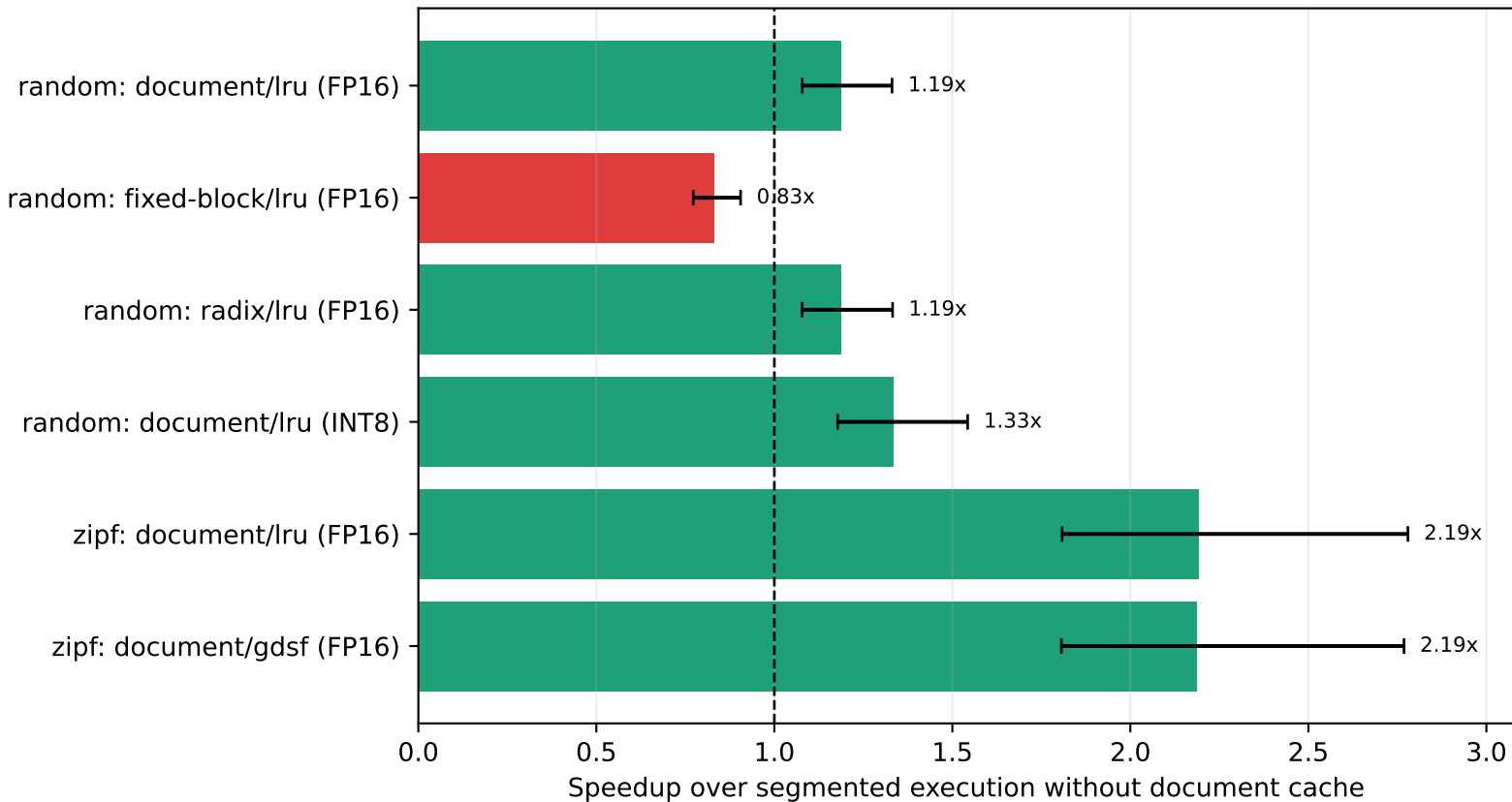
Cross-request article-KV reuse benefit (95% paired bootstrap CI)
