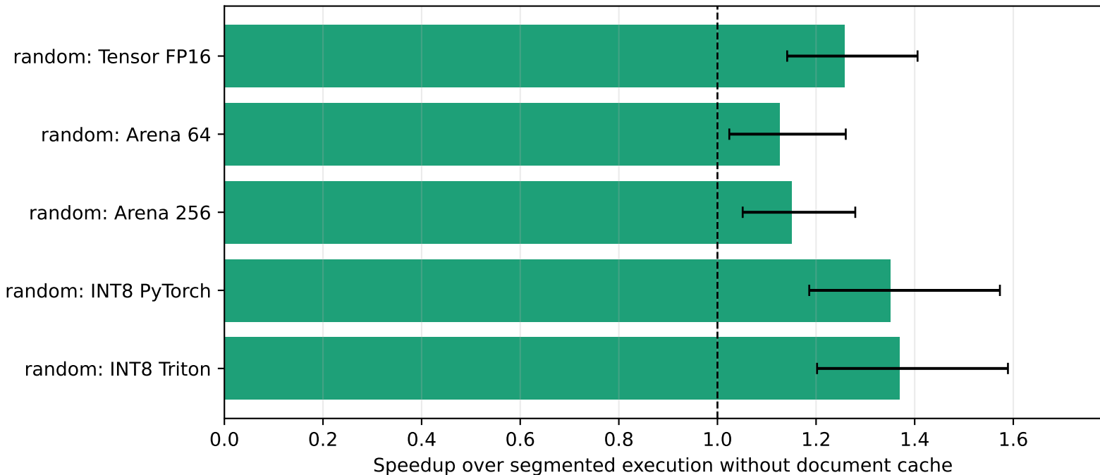
Cross-request article-KV reuse benefit (95% paired bootstrap CI)
