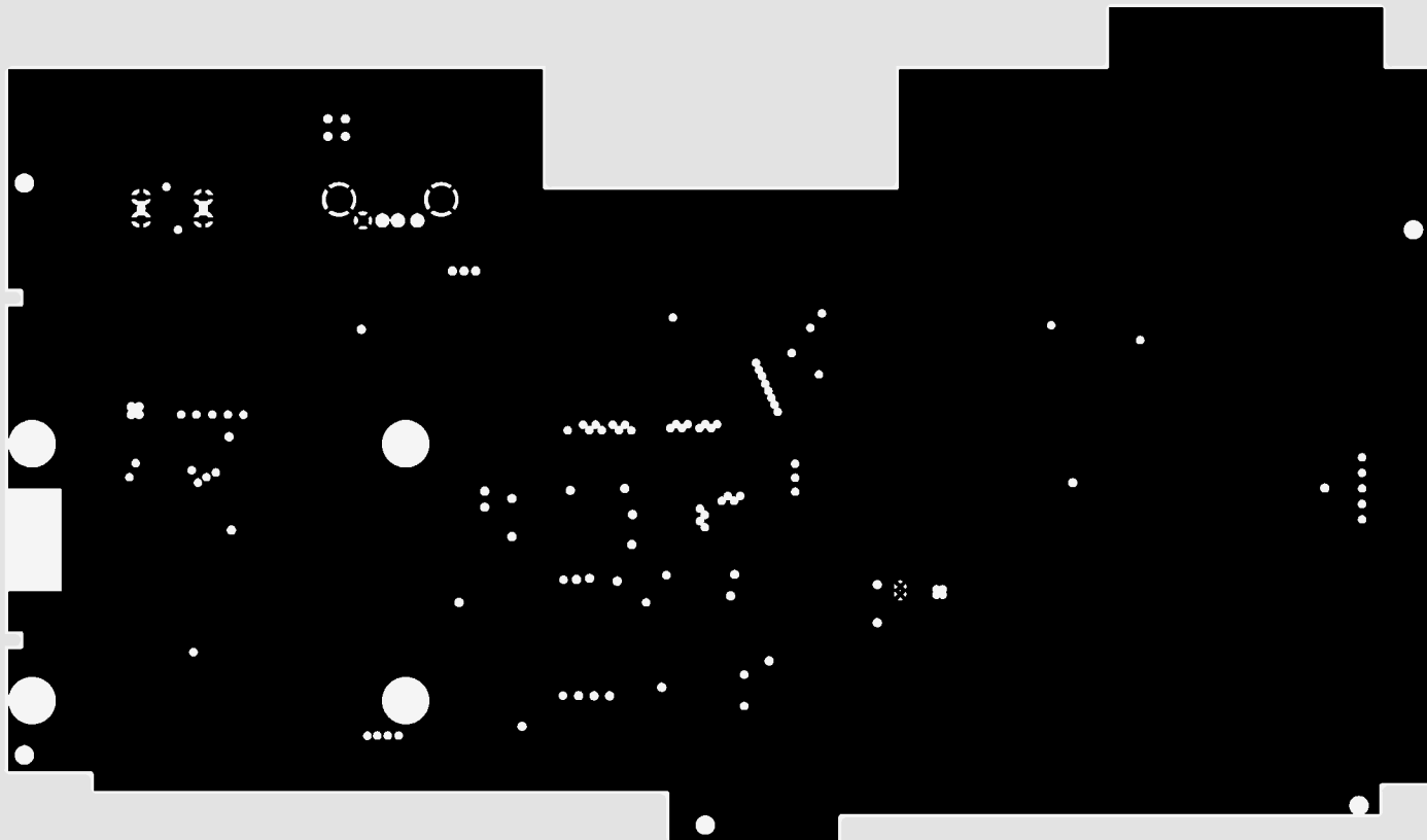
E1708058 Innerlayer 2 Image (topview)
