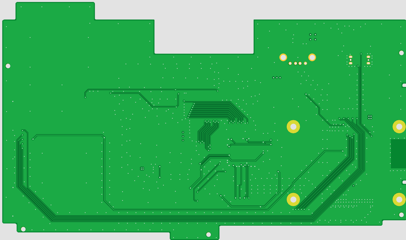
E1708058 PCB view BOTTOM (bottomview)
