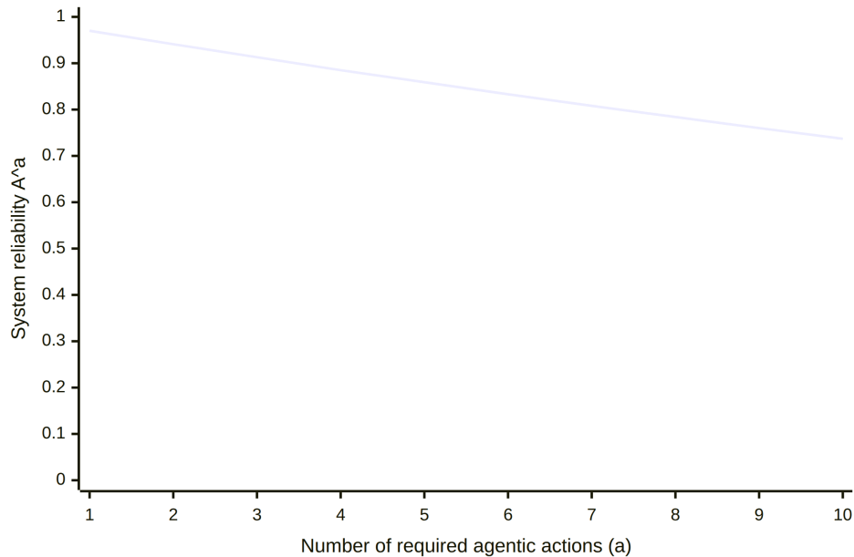
Figure 8. Statement 6 made visible. A single step at 0.97 looks reliable; the curve is what “count occurrences, not component types” means. Five required actions already sit at ~0.86, ten below 0.74 – each added exposure is a multiplication, not an addition.
