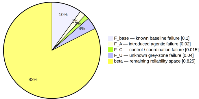
Figure 11. The partition of §13.1–§13.2: F_{base} + F_A + F_C + F_U + \beta = 1 . The known system failure F_S is the first three slices; F_U is the grey zone that exists at T_0 already; \beta (the large slice) is the capacity not yet spent on failure. The discipline is to spend \beta deliberately rather than let F_U quietly consume it.
