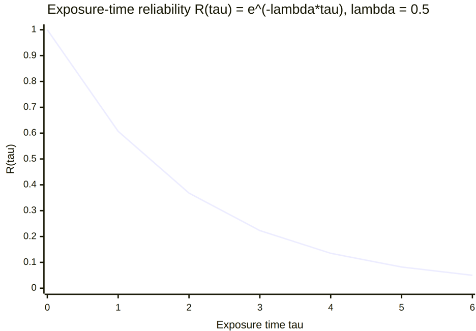
Figure 15. The constant-failure-rate model of §19.2. Because the curve is convex, cutting exposure time \tau moves reliability up the steep left part of the curve. This is the reliability sense of “faster”: less time spent in a state where failure can arrive, distinct from the throughput sense in §19.1.
