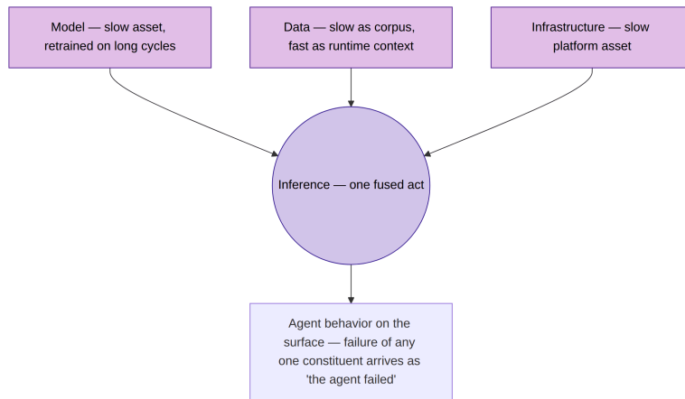
Figure 4. The dependency triangle of §4. Three things Brand would place on different layers fire together at inference time. Their reliability cannot be decomposed and re-multiplied; the fusion is what is reliable or not, and it has to be observed where it arrives.
