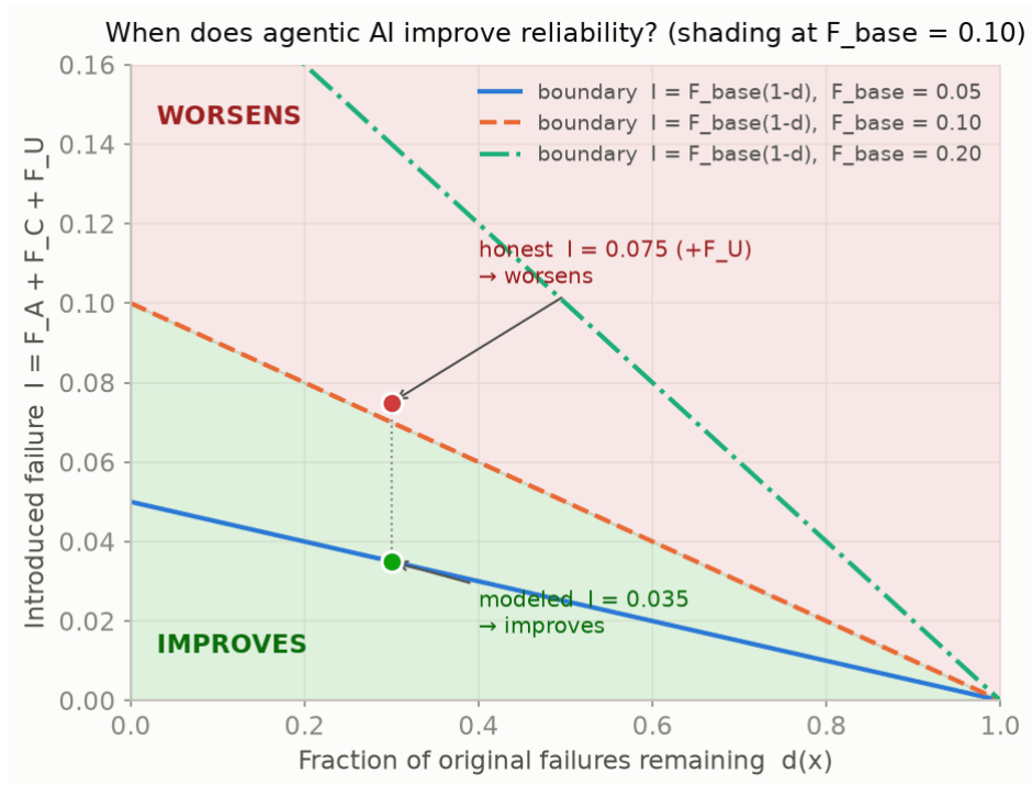
Figure 10. The improvement condition as a map. The horizontal axis is the fraction of baseline failure that survives, d(x) ; the vertical axis is the total introduced failure I = F_A + F_C + F_U . Each line is the break-even boundary I = F_{base}(1-d) for one baseline; below a line the agentic system improves reliability, above it the system worsens. The two markers replay the §11 worked example at d = 0.30 : the modelled introduced failure (0.035) sits in the improve region, but adding the honest F_U lifts I to 0.075 – across the F_{base} = 0.10 boundary into “worsens”. The honesty flip of §11 is exactly this boundary crossing.
