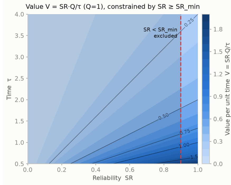
Figure 17. The compressed metric V = SR \cdot Q / \tau (with Q = 1 ) drawn as a field over reliability and time. Value grows toward the bottom-right – high SR , low \tau – and the diagonal contours are lines of equal value, so a fast unreliable system and a slow reliable one can share one. The constraint of Statement 21 is the vertical cut: everything to the left of SR_{min} is inadmissible however high V climbs, which is why value optimization must be constrained, not maximized freely.
