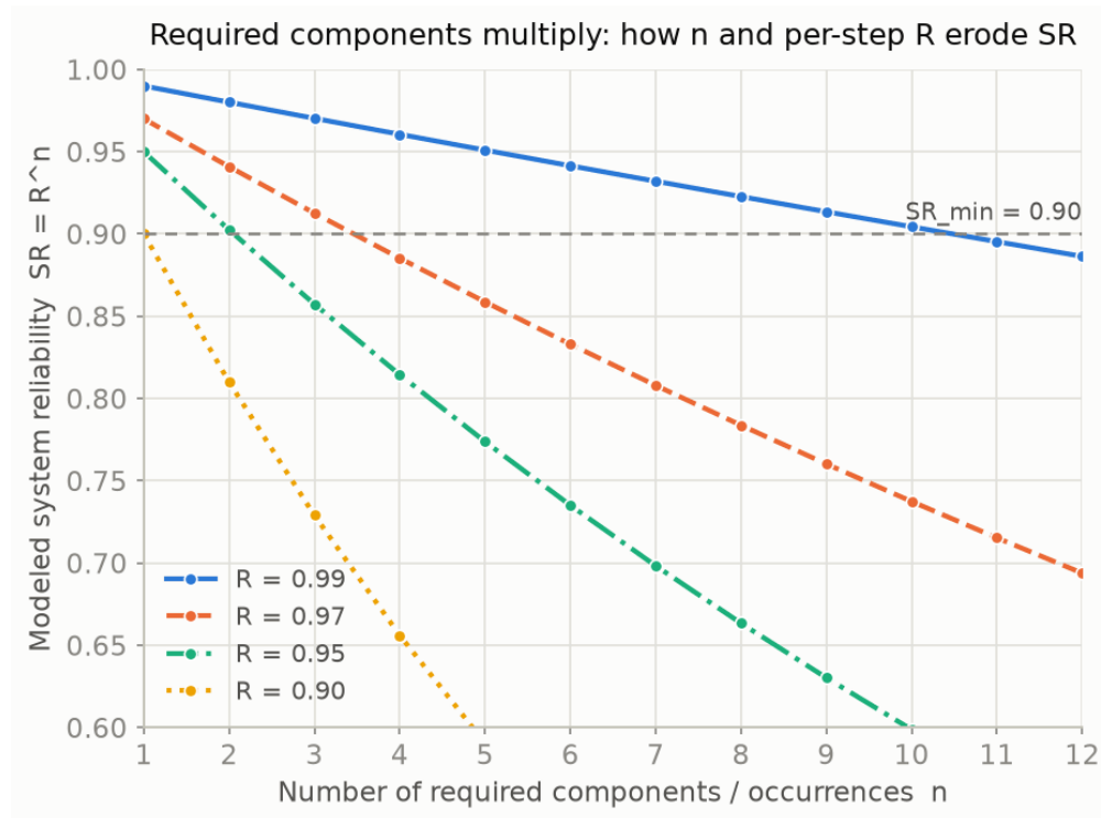
Figure 5. How the product SR = \prod_{i=1}^n R_i behaves when n identical required components each have reliability R . Each curve fixes one value of R ; the dashed line is an illustrative floor SR_{min} = 0.90 . Components that look reliable in isolation still fall through the floor as occurrences accumulate – even R = 0.97 crosses it by the fourth required step. This is the visual form of Axiom 2: every required dependency weakly reduces reliability, and the reduction compounds.
