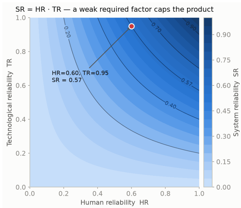
Figure 2. The full response surface behind Figure 1. Colour is SR = HR \cdot TR over every combination of the two required factors; the curved lines are contours of constant SR , and the 0.57 contour runs through the worked point (0.60, 0.95). The shape is the whole point: raising the strong factor slides you along a contour, not up it – only lifting the weaker factor moves SR upward.
