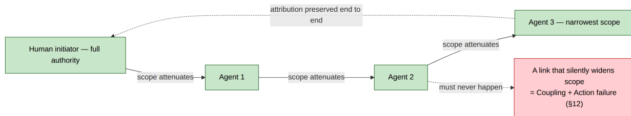
Figure 13. Multi-hop delegation. Scope must attenuate at every hop (solid arrows narrowing), and attribution must trace back to the originating human (dashed return). A middle link that widens scope or loses the originator is §12's Coupling and Action failure materialised.
