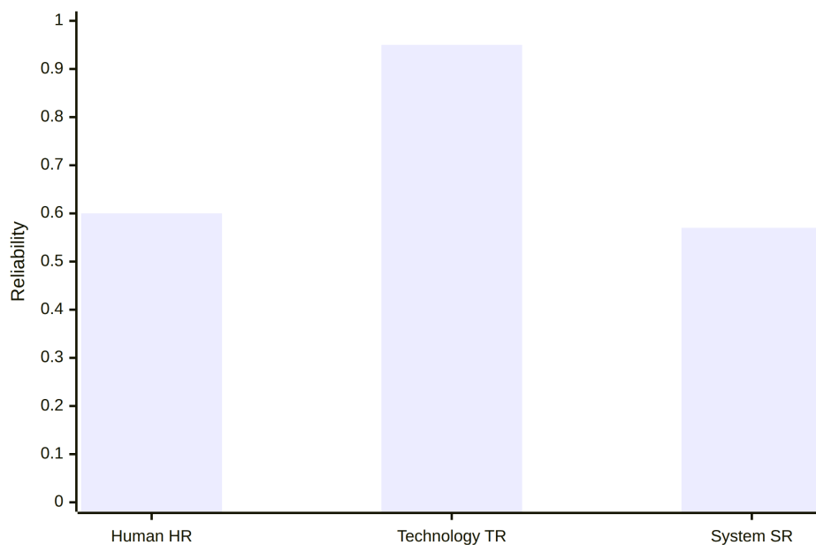
Figure 1. The multiplicative coupling of Statement 1. The system (0.57) lands below both of its required factors, not between them. A strong technical part cannot lift the product above the weak human part.
