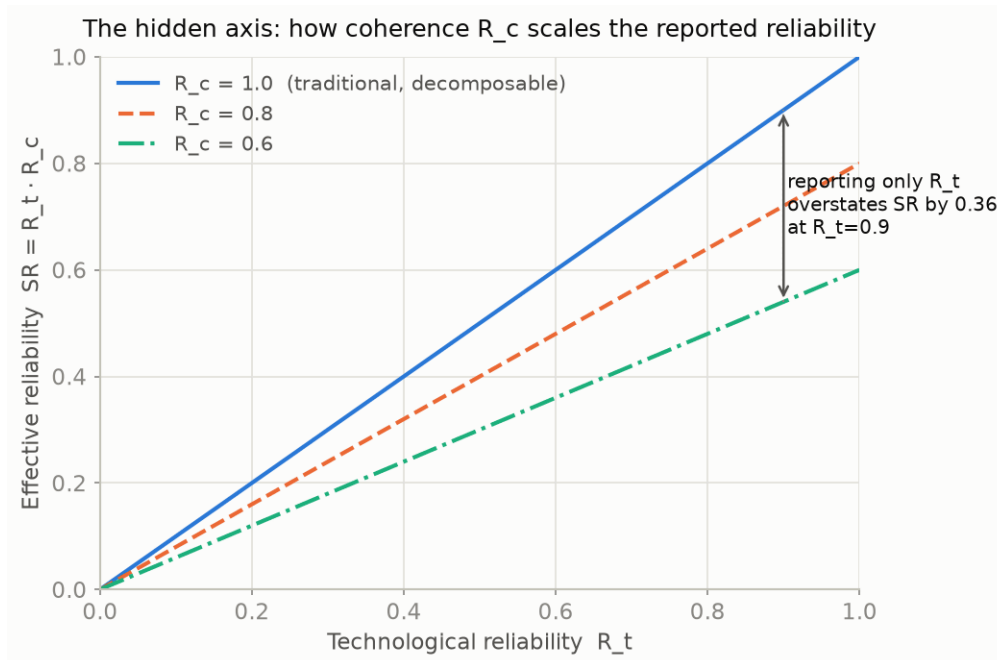
Figure 7. The multiplicative cost of the coherence axis, drawn as the product R_t \cdot R_c . Each line fixes R_c and sweeps R_t . Traditional decomposable systems ride the top line
