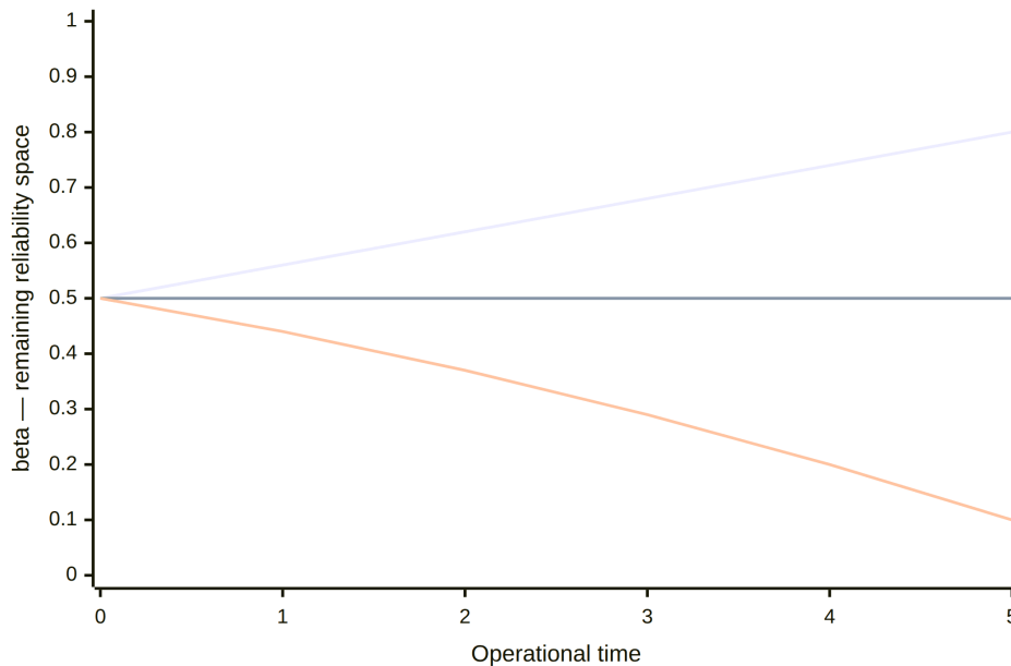
Figure 12. Statement 13 across time, three lines from a shared starting \beta . Top: E_{in} > E_{entropy} – surplus maintenance pays down debt and \beta grows (left column of the table). Middle: E_{in} = E_{entropy} – breakeven, \beta flat but fragile. Bottom: E_{in} < E_{entropy} – entropy wins, \beta shrinks invisibly while roadmaps still look good, until F_U dominates.
