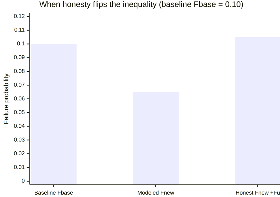
Figure 9. The §11 worked example. On modeled terms the agentic system improves ( 0.065 < 0.10 , second bar below the baseline line). Add the unmodeled exposure F_U that §12 insists on naming and the same system crosses back above baseline ( 0.105 > 0.10 ). The arithmetic is honest only when every term is on the page.
