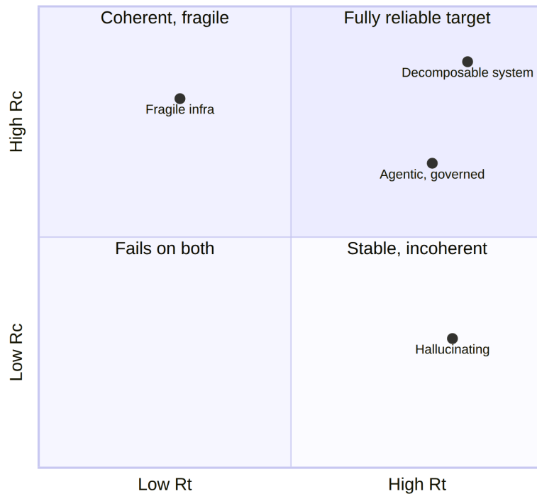
Figure 6. The two axes of Statement 5. Traditional engineering lives on the top edge where R_c = 1 and the scalar model is exact. Agentic systems drop off that edge; a high- R_t system that hallucinates (bottom-right) and a coherent system on fragile infrastructure (top-left) are different failures, and reporting only R_t hides one of them.
