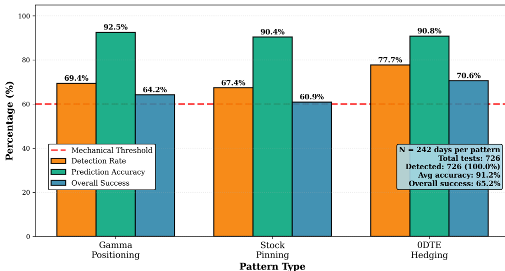
Pattern Detection Performance Metrics (Unbiased Prompts, Full 2024)
