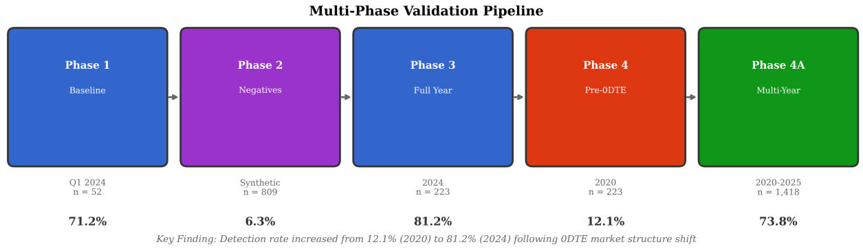
Fig. 4. Multi-Phase Validation Pipeline. Detection rates progressed from Phase 1 baseline (71.2%) through negative controls (6.3%), full 2024 validation (81.2%), and 2020 pre-ODTE comparison (12.1%).
