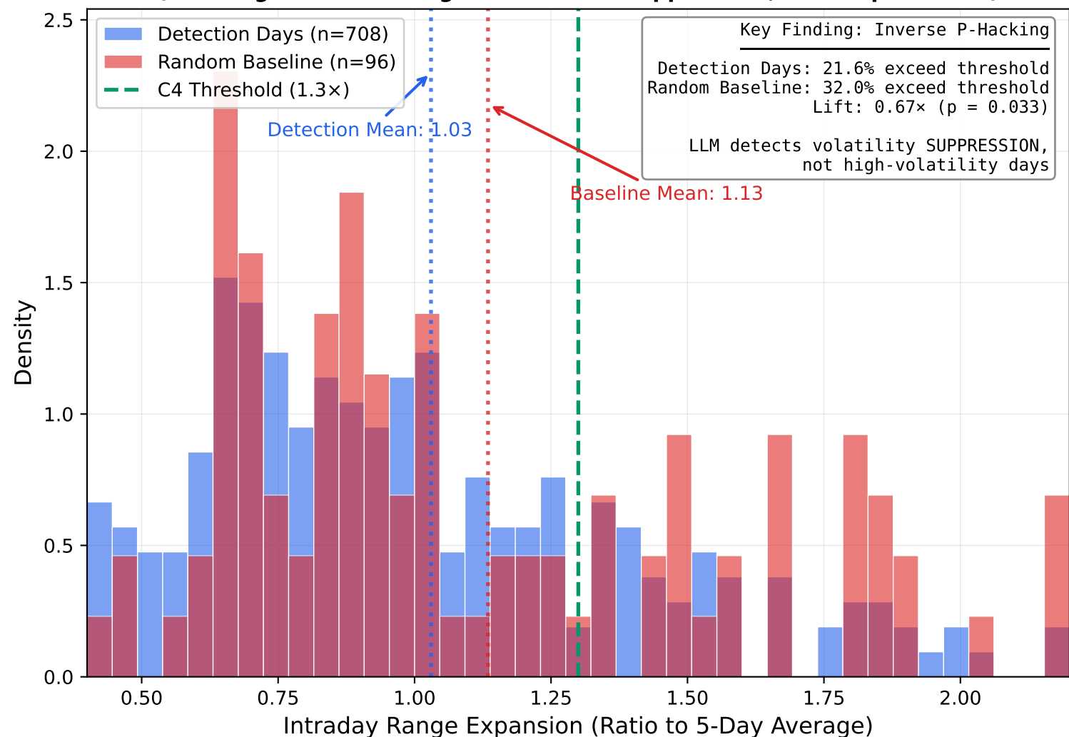
Figure 4: Detection Days Show LOWER Range Expansion Than Baseline (Proof Against P-Hacking: LLM Detects Suppression, Not Amplification)
