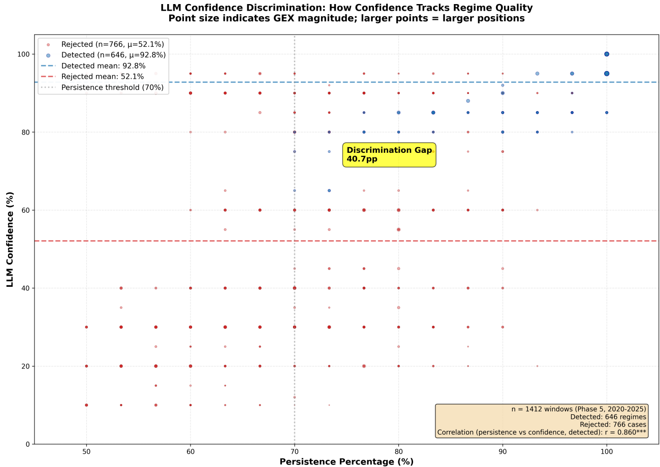
Fig. 7. LLM Confidence Discrimination Across Full Detection Spectrum. Scatterplot showing relationship between persistence (X-axis) and LLM confidence (Y-axis) for all 1,412 Phase 5 windows. Blue points represent detected regimes ( n=646 , mean confidence 92.8%), red points represent rejected cases ( n=766 , mean confidence 52.1%). Point size encodes GEX magnitude (larger points indicate larger dealer positions). The 40.7 percentage point confidence gap demonstrates strong discrimination between regimes and non-regimes. Persistence threshold line (vertical dotted) at 70% shows where regime classification criterion is applied. Strong correlation between persistence and confidence ( r = +0.860 ) for detected regimes indicates confidence meaningfully tracks regime strength.
