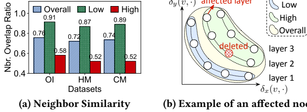
Figure 7: Neighbor similarity of affected nodes before and after reinsertion-based repair.
