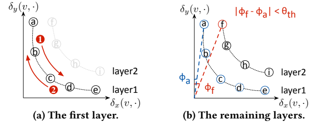
Figure 6: Illustration of ACAR.
