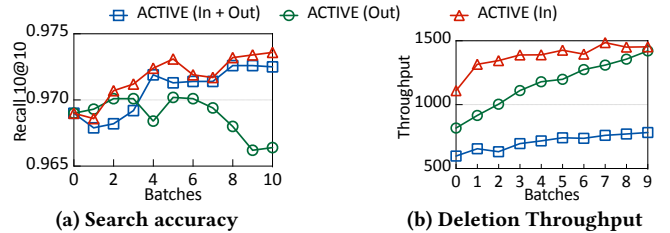
Figure 20: Impact of different affected node definitions.
