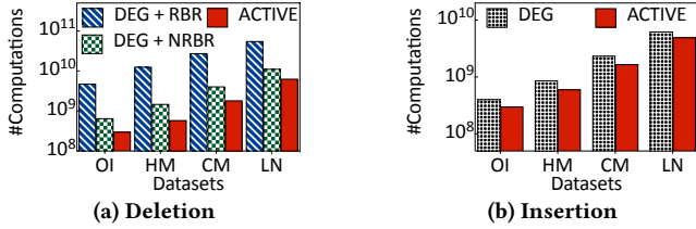
Figure 12: Distance computation comparison.
