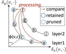
Figure 4: Illustration of the existing AR computation algorithm [56].
