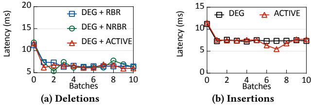
Figure 15: Search latency comparison.
