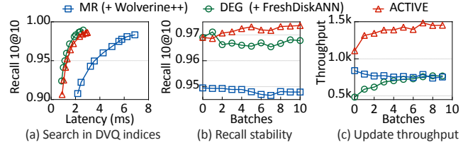
Figure 1: Performance of DVQ indices under static search and dynamic updates on the OpenImage dataset, where “MR” denotes multi-index retrieval.
