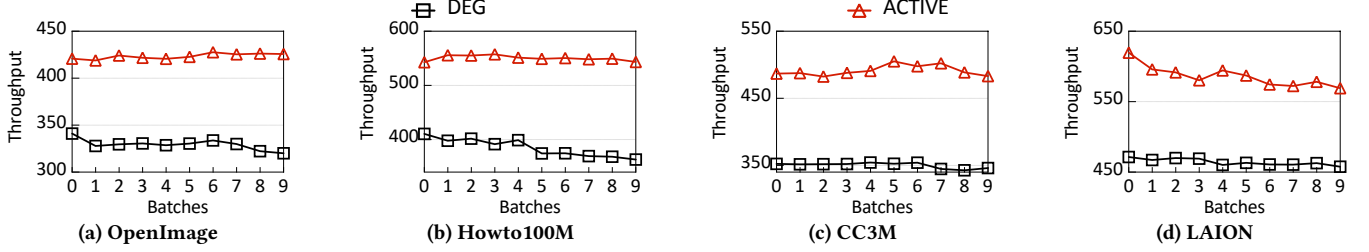
Figure 11: Throughput comparison under insertions.
