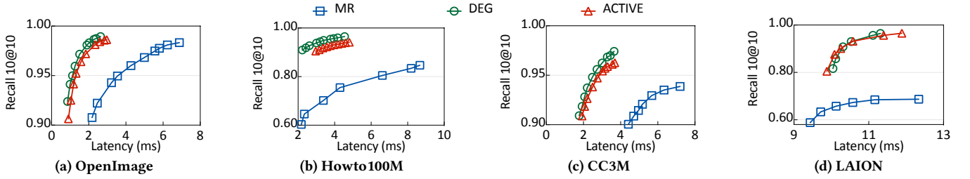
Figure 9: Comparison of the trade-offs between search accuracy and latency. The top left is better.
