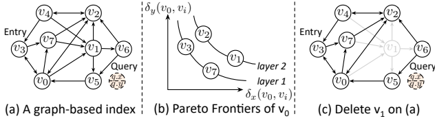
Figure 2: An example of a graph-based DVQ index. Each node maintains at most R = 4 neighbors. The dashed circle indicates a dual-vector query, v_3 is the entry node, and v_5 is the node most similar to the query under the given preference.
