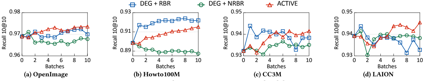
Figure 13: Search accuracy comparison under deletions.
