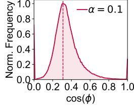
Figure 5: Distribution of retrieved nodes across different Pareto angles \phi .
