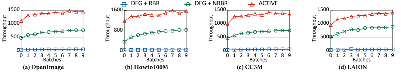
Figure 10: Throughput comparison under deletions.
