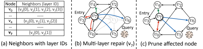
Figure 8: An illustrative example of multi-layer repair.
