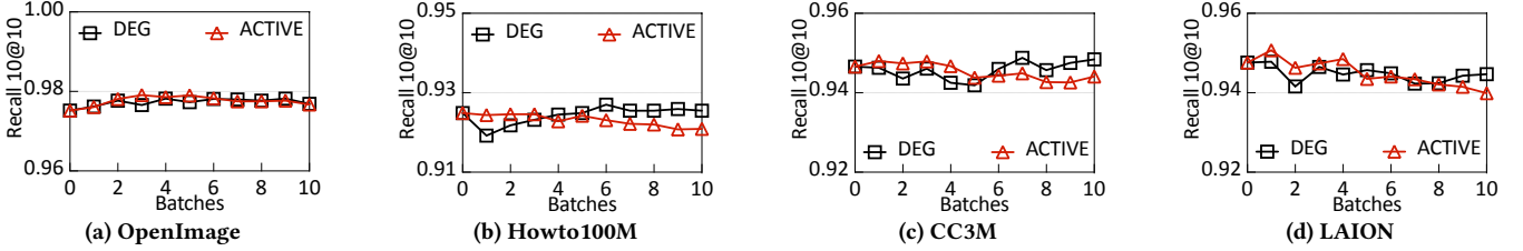
Figure 14: Search accuracy comparison under insertions.
