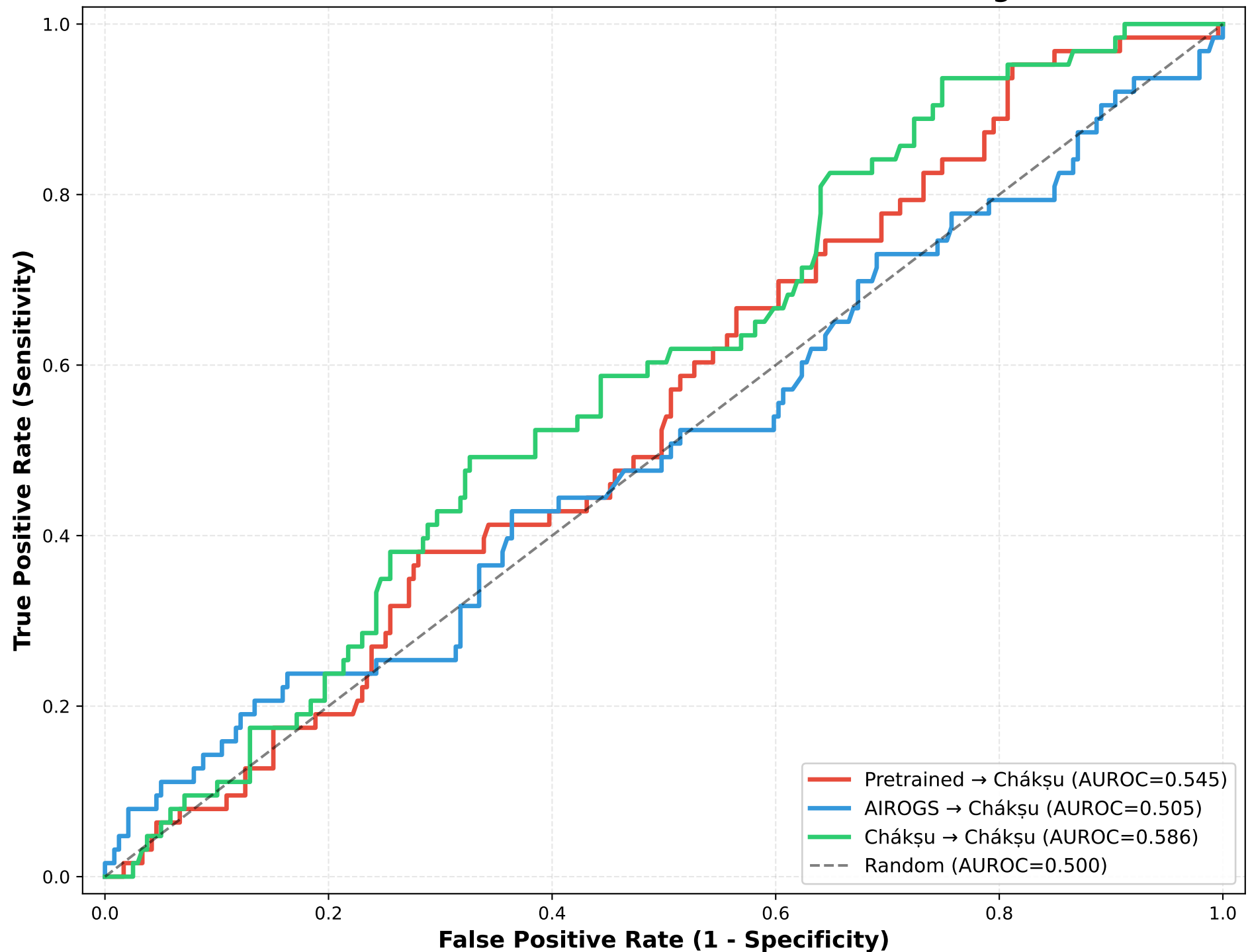
ROC Curves: Cross-Ethnic Glaucoma Screening
