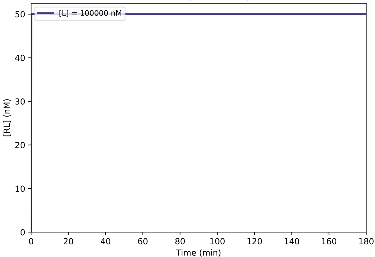
Binding kinetics -- [RL](t) (dashed = analytical steady state)
