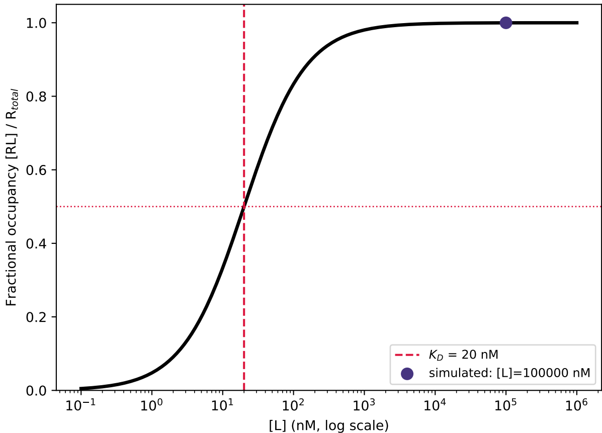
Dose-response (Hill-Langmuir, n = 1 )
