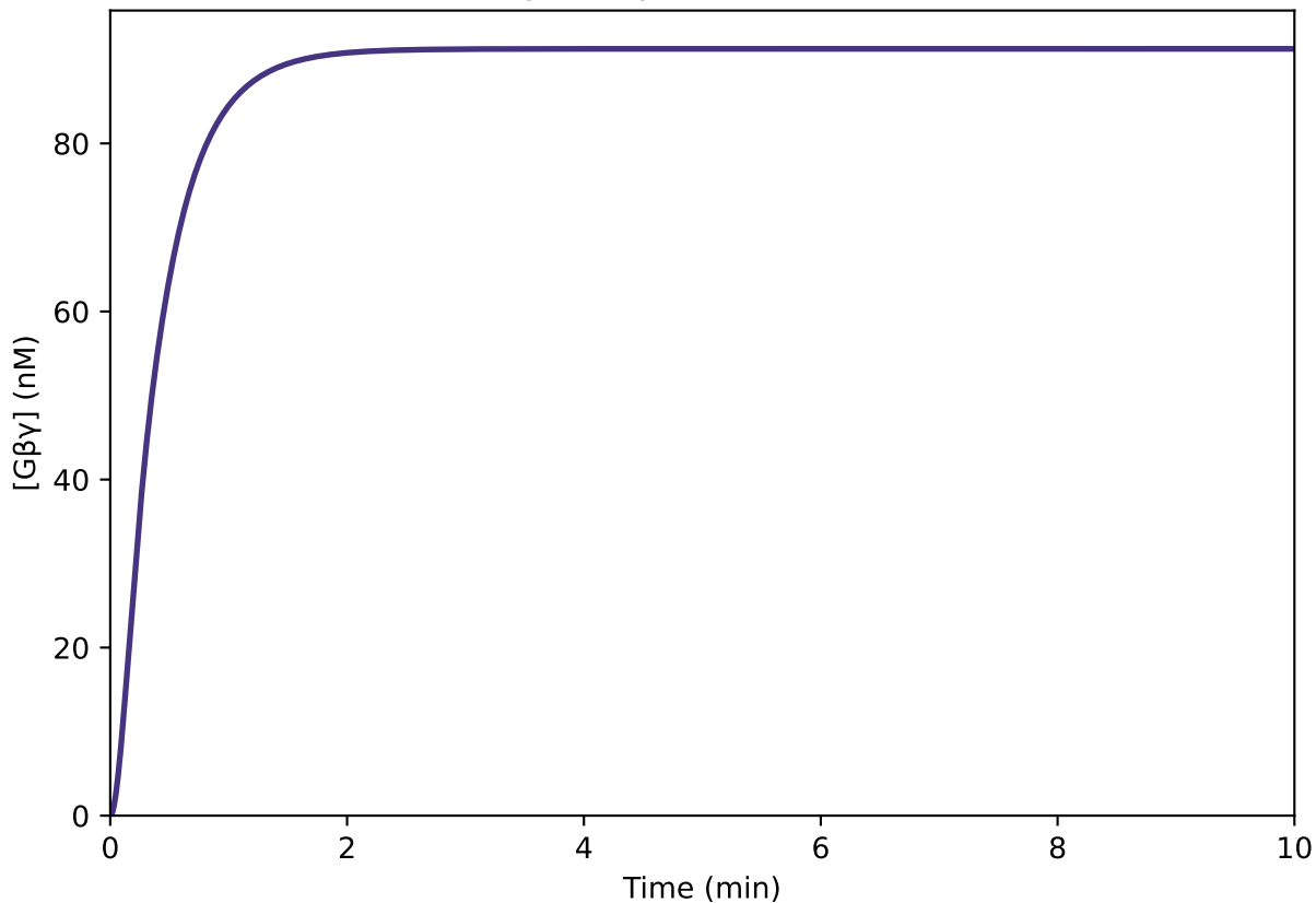
Free G\beta\gamma over time (signal input to Module 3)
