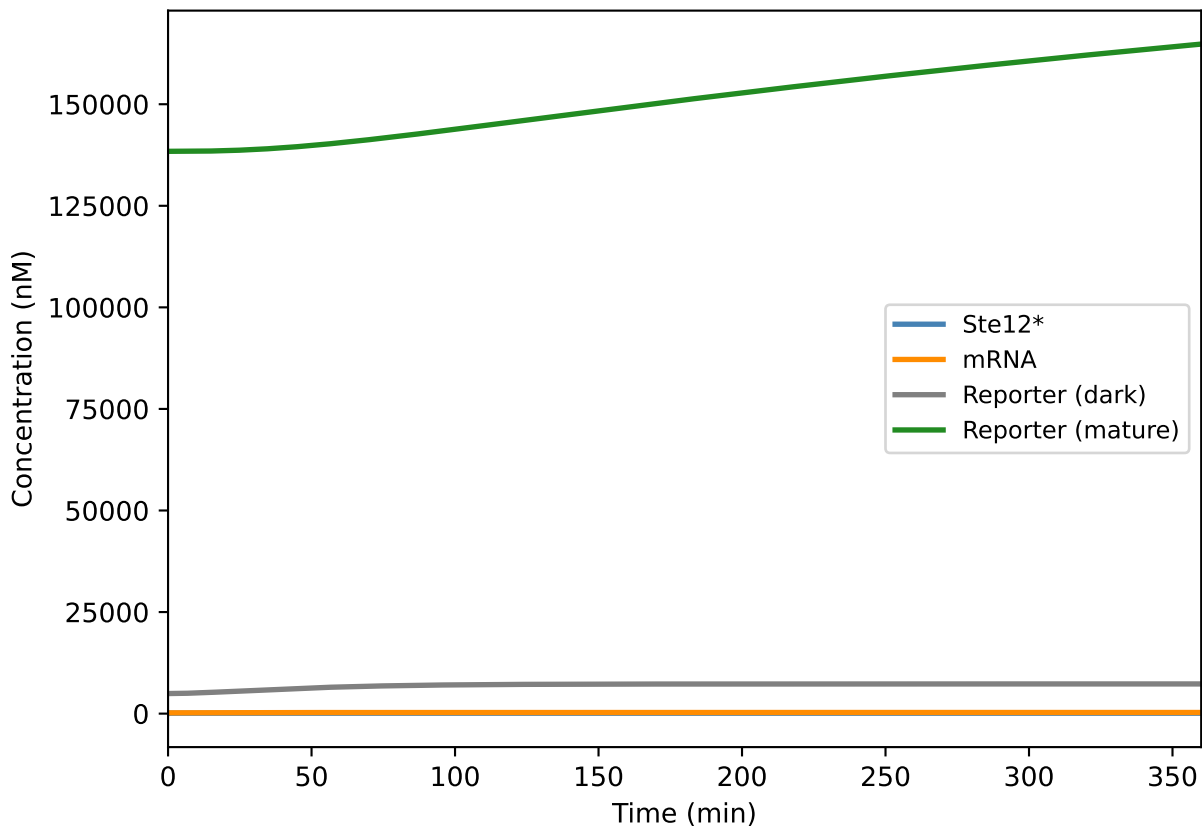
All four species ([L] = 100000 nM, wet-lab dose)
