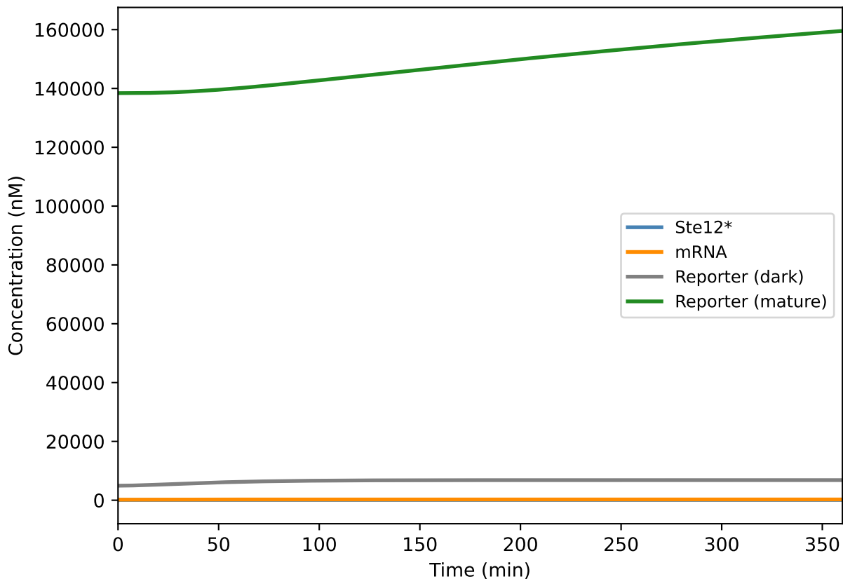
All four species (v2) ([L] = 100000 nM, wet-lab dose)
