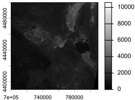
Green
