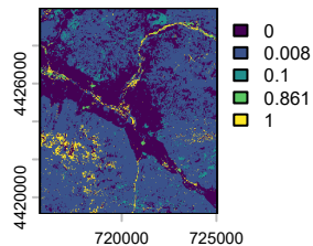
willow
