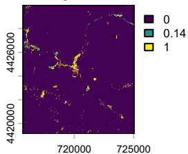
hydric
