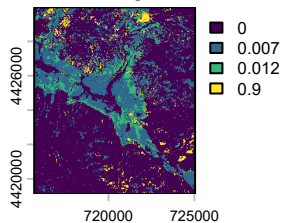
rocky
