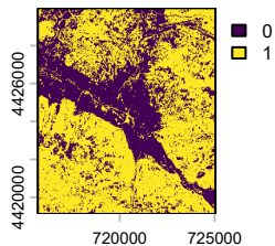
forest
