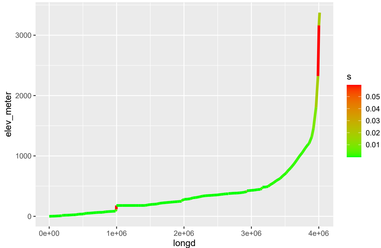
Nile River to Blue Nile longitudinal profile
