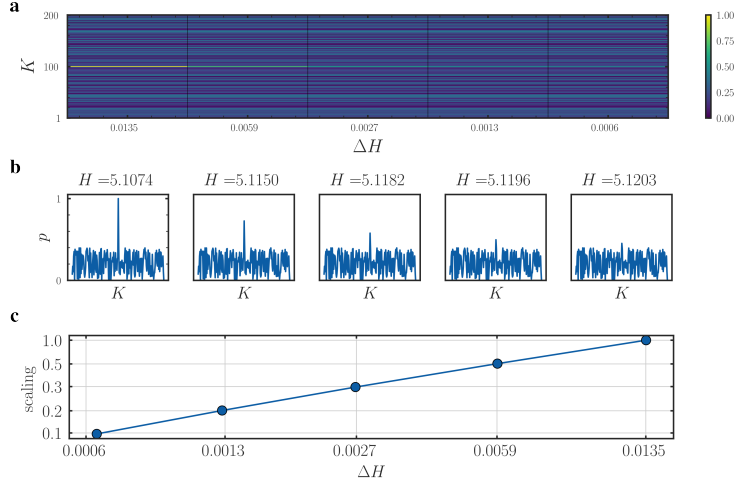
Figure 9: SHOWCASE OF DISTRIBUTION ENTROPY - a : visualization of each distribution as heatmaps (columns), the entropy differences (x-axis) and arm indexes (y-axis); note that the entropy of distribution i is inversely proportional to the difference \Delta H - b : examples of distributions for increasing levels of entropy; the reported values reference the same data of plot a - c : log-log plot of the entropy differences (x-axis) against the scaling \Delta of the top-arm with respect to the others (y-axis)
