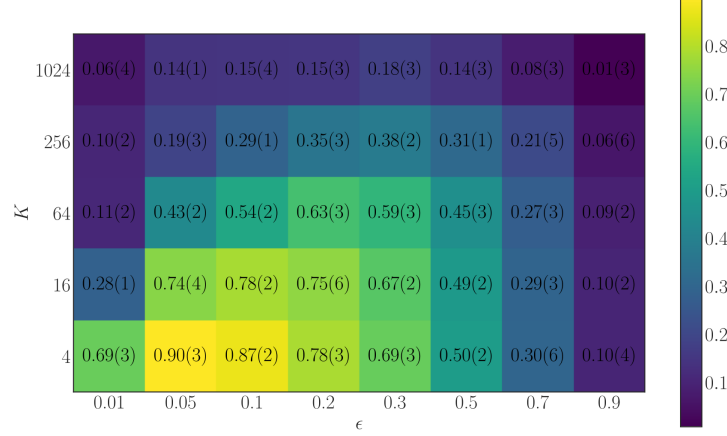
Figure 6: SENSITIVITY ANALYSIS OF EPSILON-GREEDY - performance of the algorithm on a piecewise stationary MAB for varying number of arms and \epsilon parameter. In parenthesis is reported the decimal position of the first significant digit.
