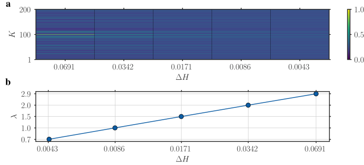
Figure 10: SHOWCASE OF DISTRIBUTION ENTROPY - a : visualization of each distribution as heatmaps (columns), the entropy differences (x-axis) and arm indexes (y-axis); note that the entropy of distribution i is inversely proportional to the difference \Delta H - b : log-log plot of the entropy differences (x-axis) against the scaling \lambda of the top-arm with respect to the others (y-axis).
