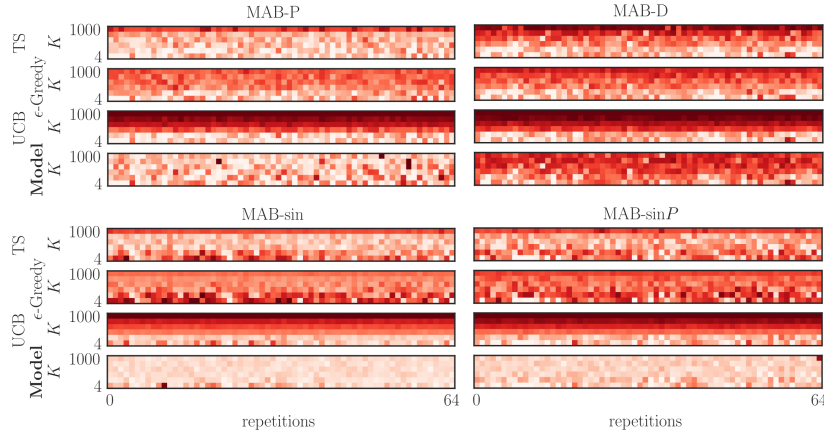
Figure 9: HEATMAP OF MULTIPLE RUNS - Each single heatmap shows the average regret (white=low, dark red=high) of two trials for a single model on a given environment for a specific number of arms K .
