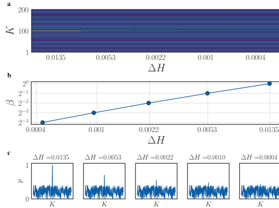
Figure 8: SHOWCASE OF DISTRIBUTION ENTROPY
