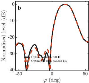
Banded-model ablation
