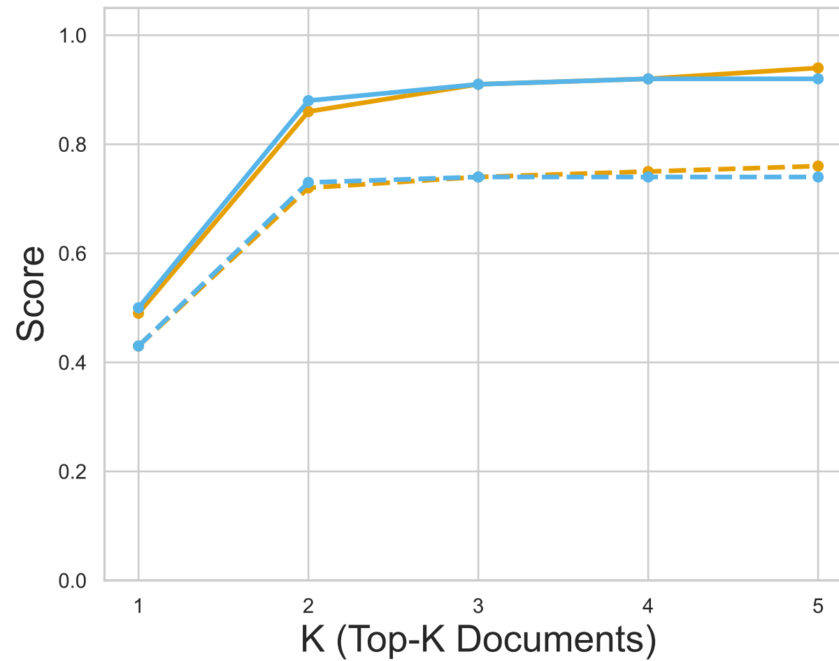
Recall@K
