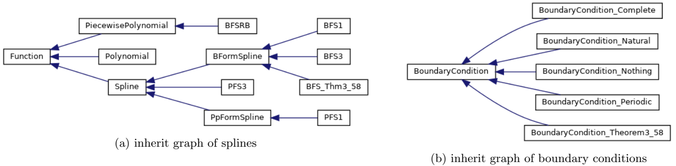
Figure 1: inherit graph
