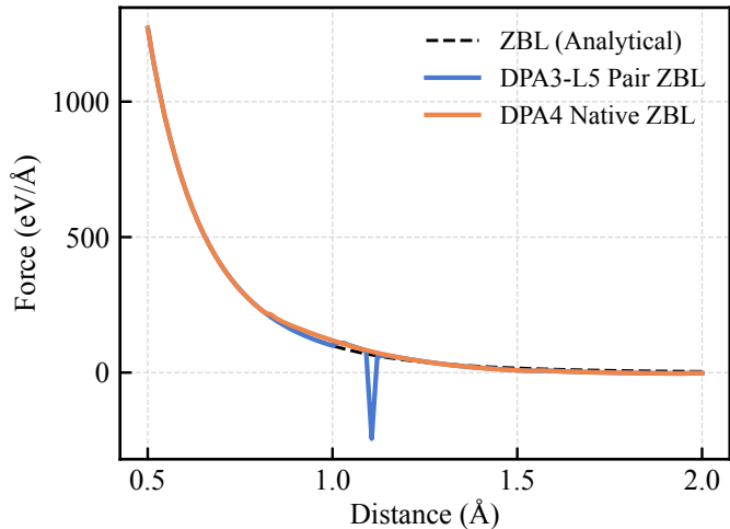
Dimer Force
