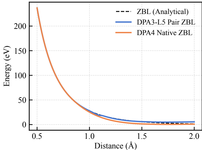
Dimer Energy
