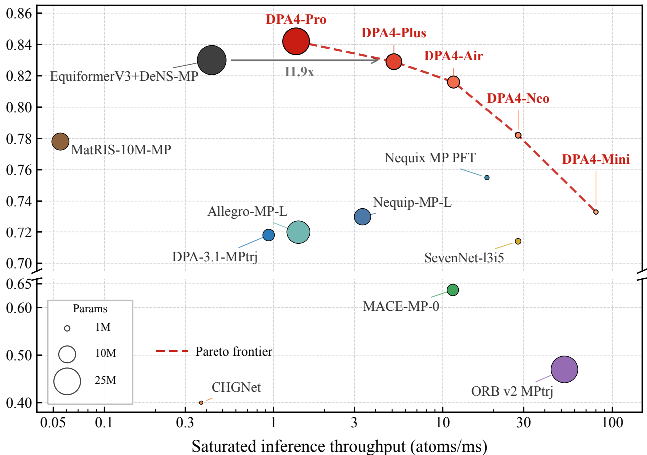
Matbench Discovery CPS
