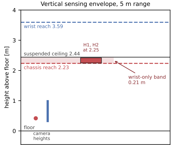
Fig. 3. Why exactly two changes are unreachable. Sweeping all base yaws at the 5 m range limit, the highest point the chassis camera can place inside its frustum is 2.23 m; the wrist camera reaches 3.59 m (swept at 5 mm resolution). The ceiling begins at 2.44 m, leaving a wrist-only band 0.21 m tall. The two height changes sit in it at 2.25 m.
