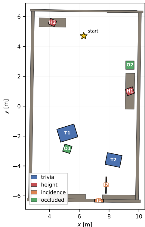
Fig. 2. Hall B, clipped from a real IFC export, with the eight injected changes coloured by observability class. Grey is the modelled shell and fit-out. The robot starts at the marked pose.
