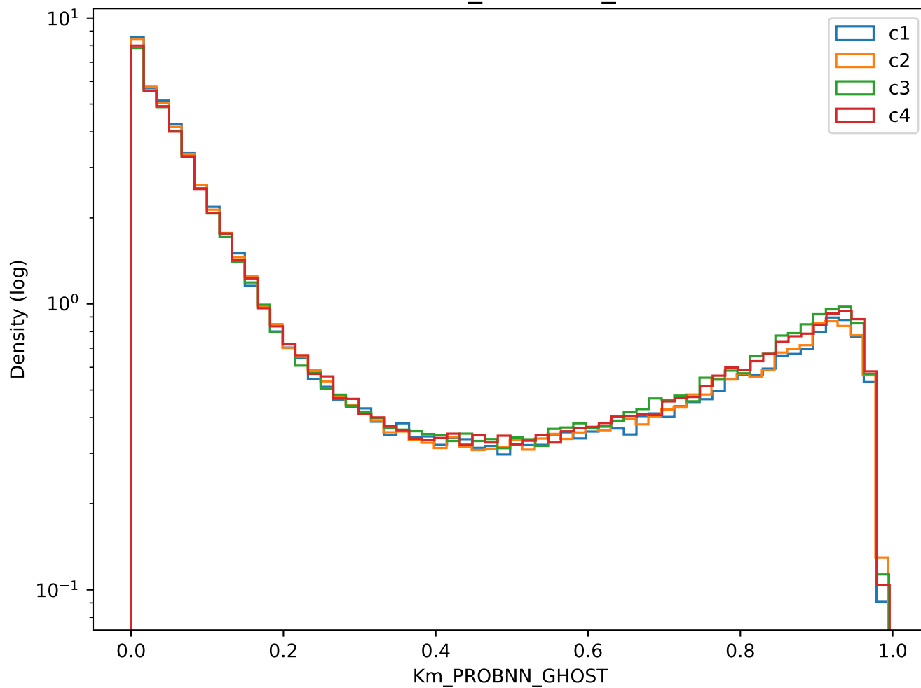
Branch: Km_PROBNN_GHOST
