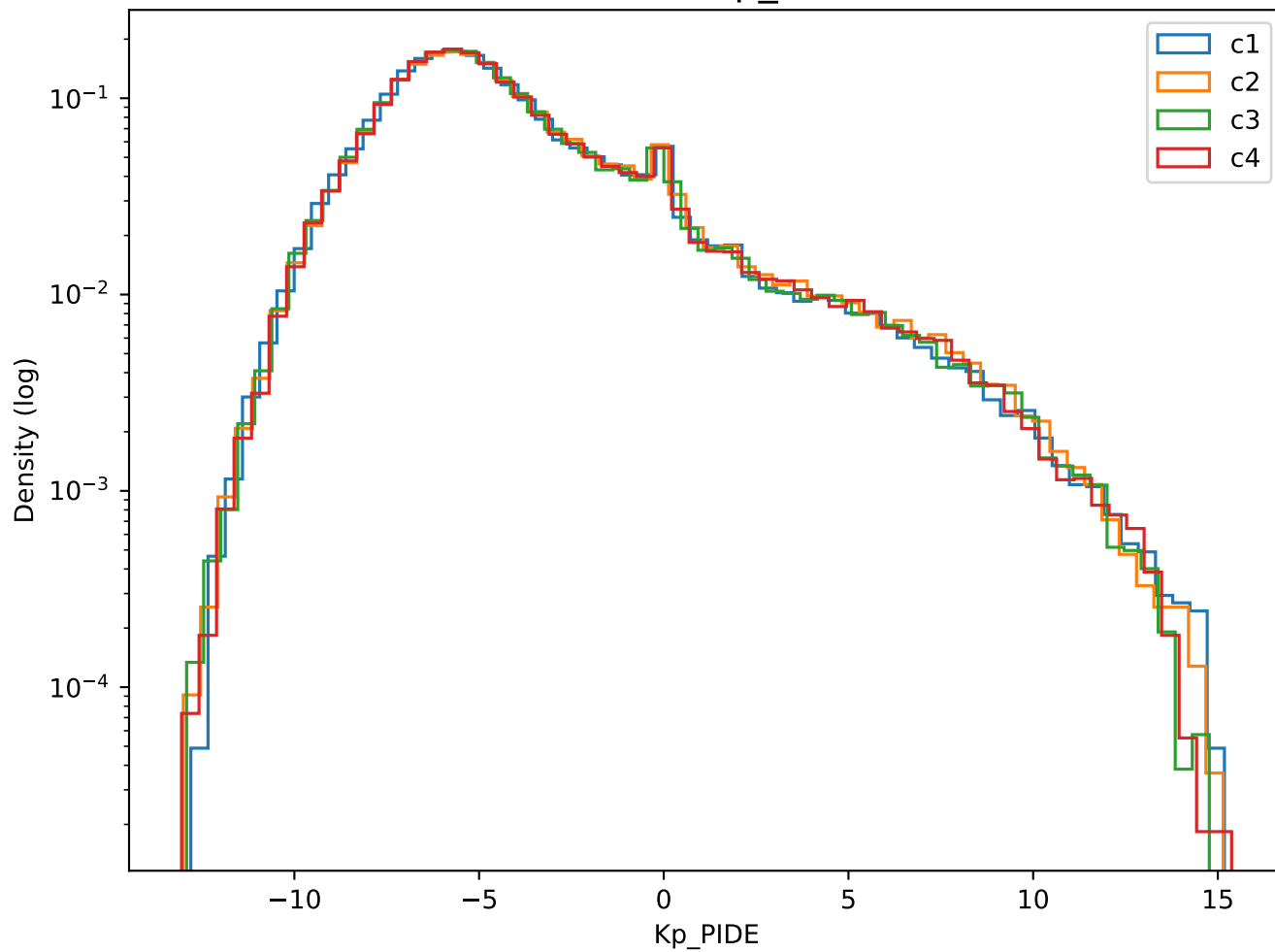
Branch: Kp_PIDE
