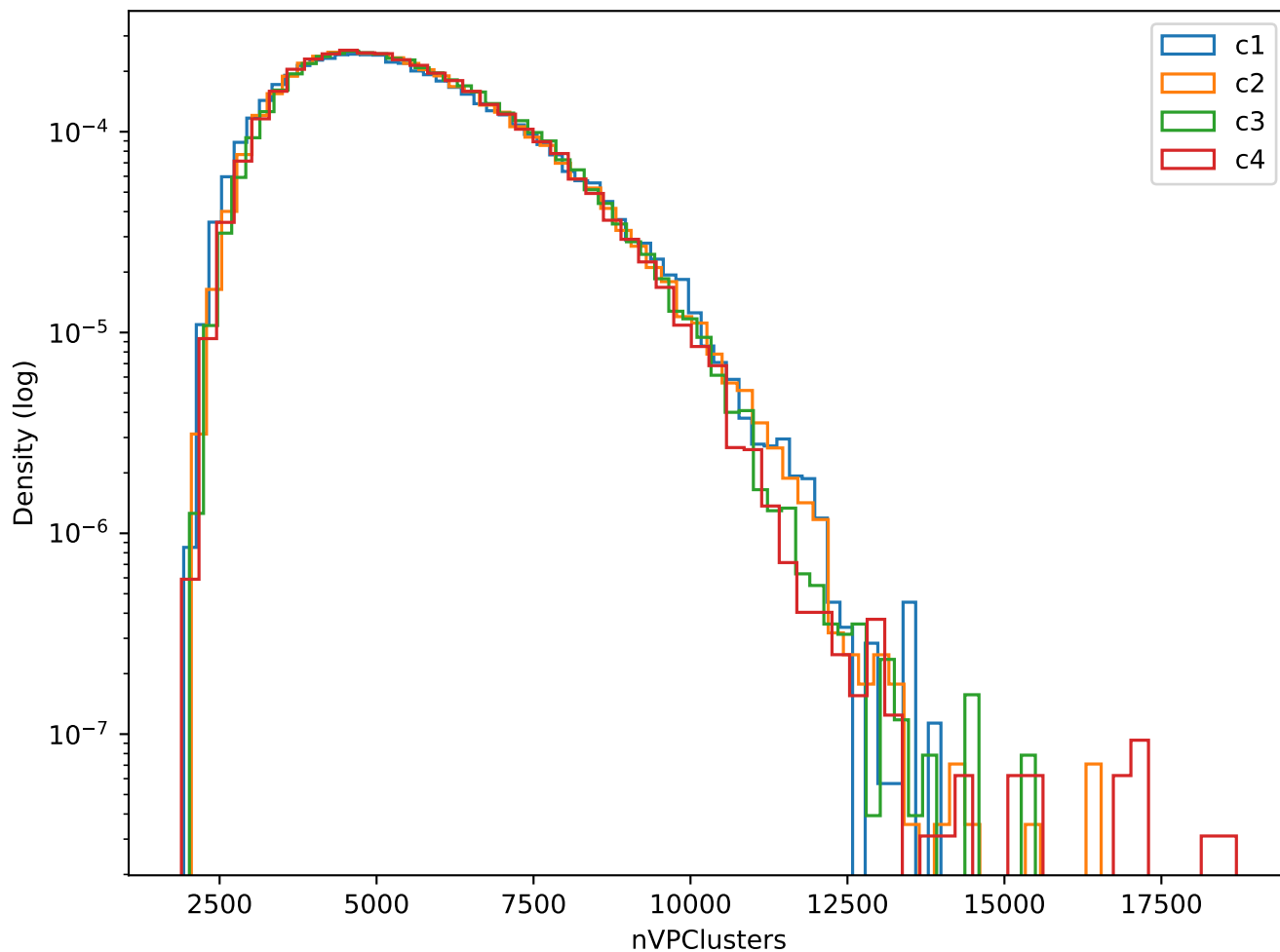
Branch: nVPClusters
