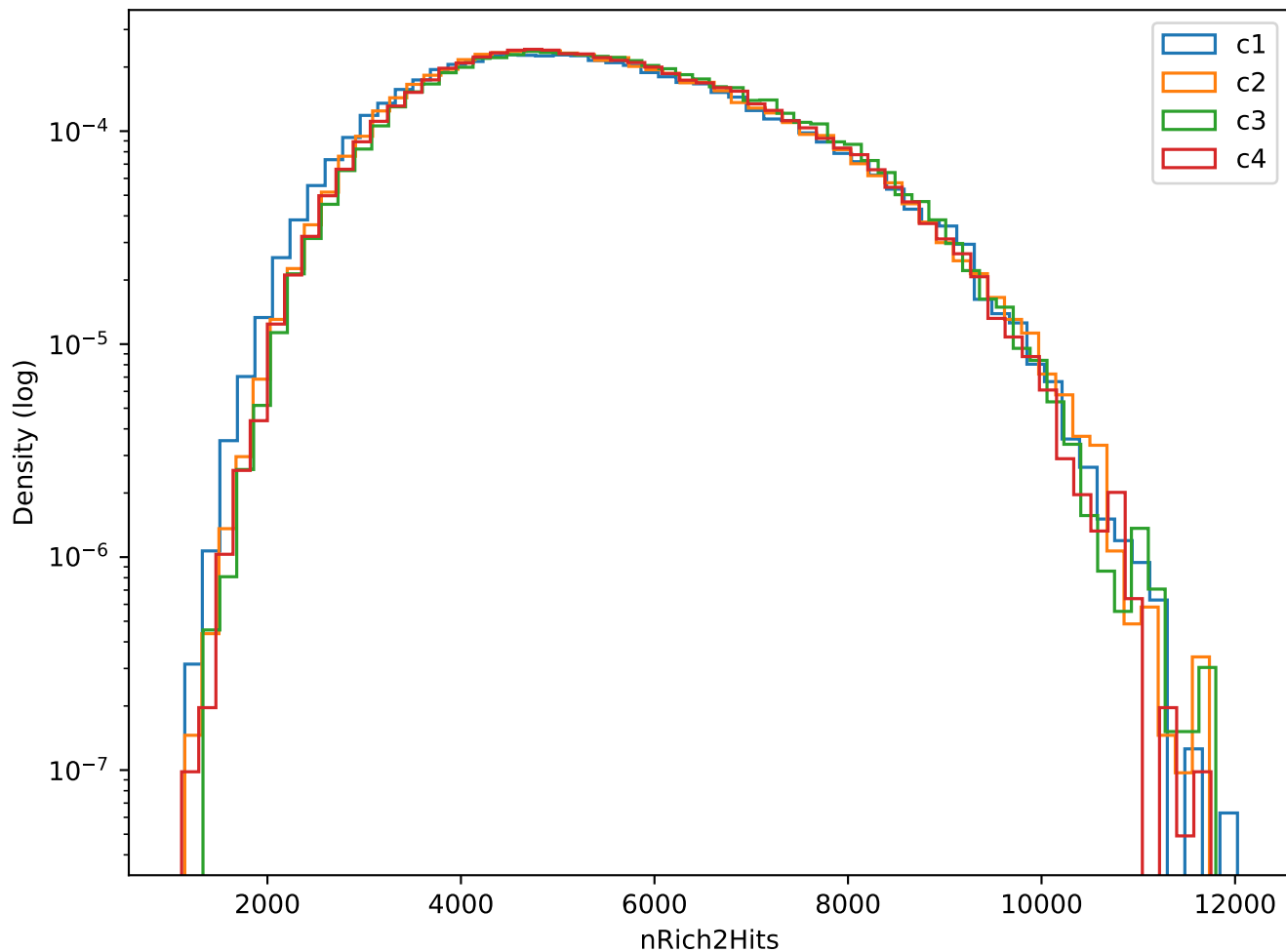
Branch: nRich2Hits
