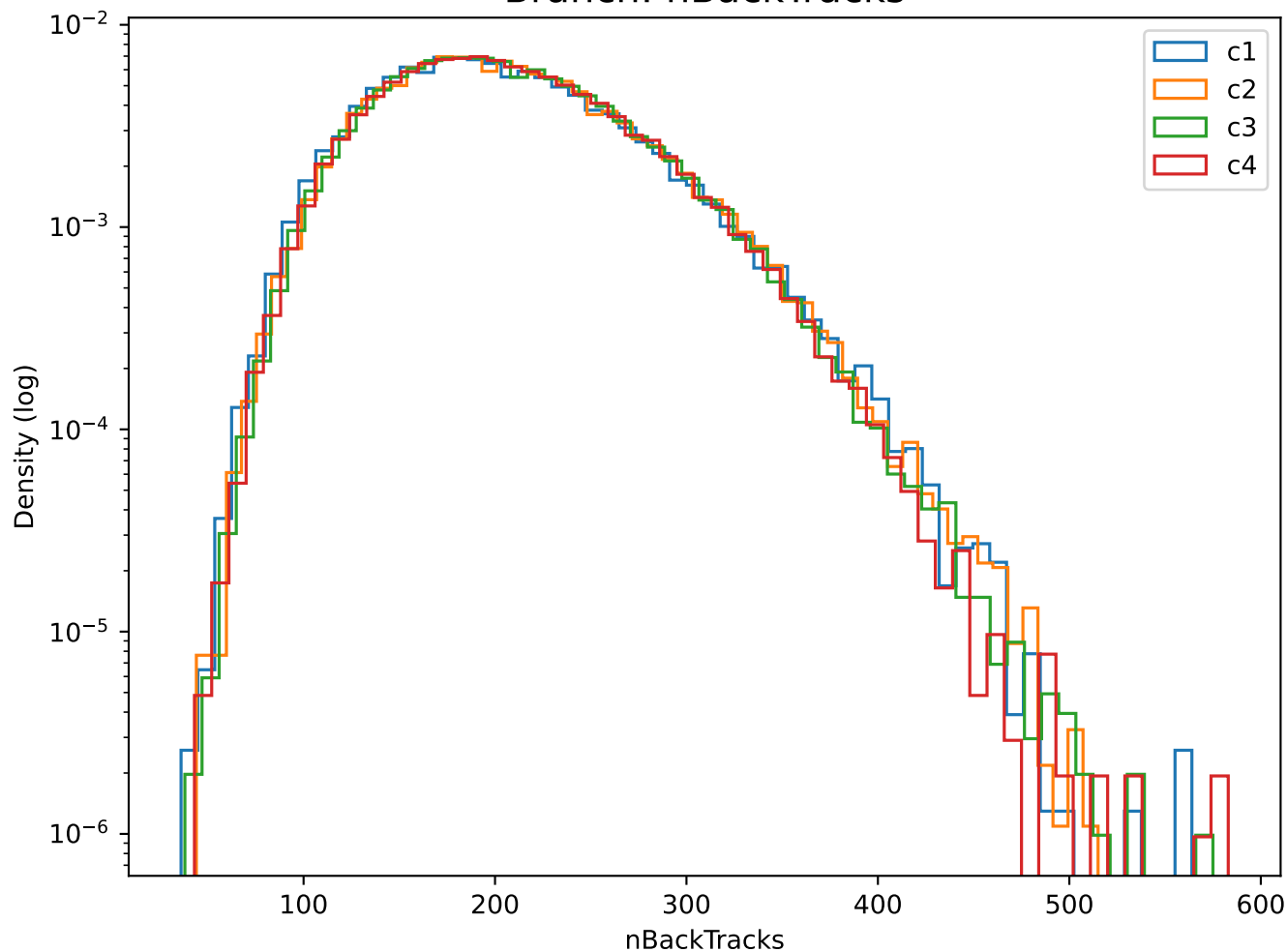
Branch: nBackTracks
