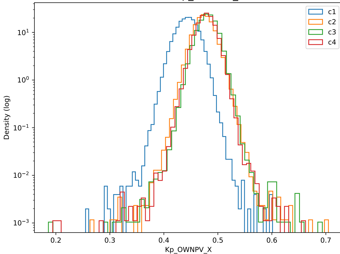
Branch: Kp_OWNPV_X
