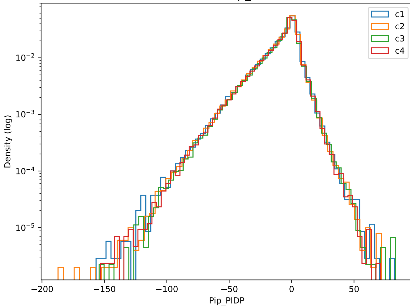
Branch: Pip_PIDP
