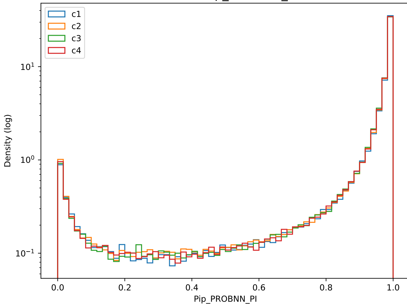
Branch: Pip_PROBNN_PI
