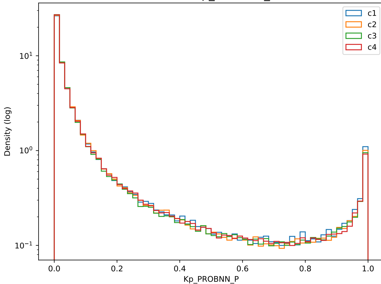
Branch: Kp_PROBNN_P
