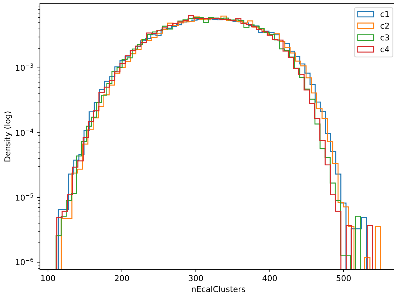
Branch: nEcalClusters
