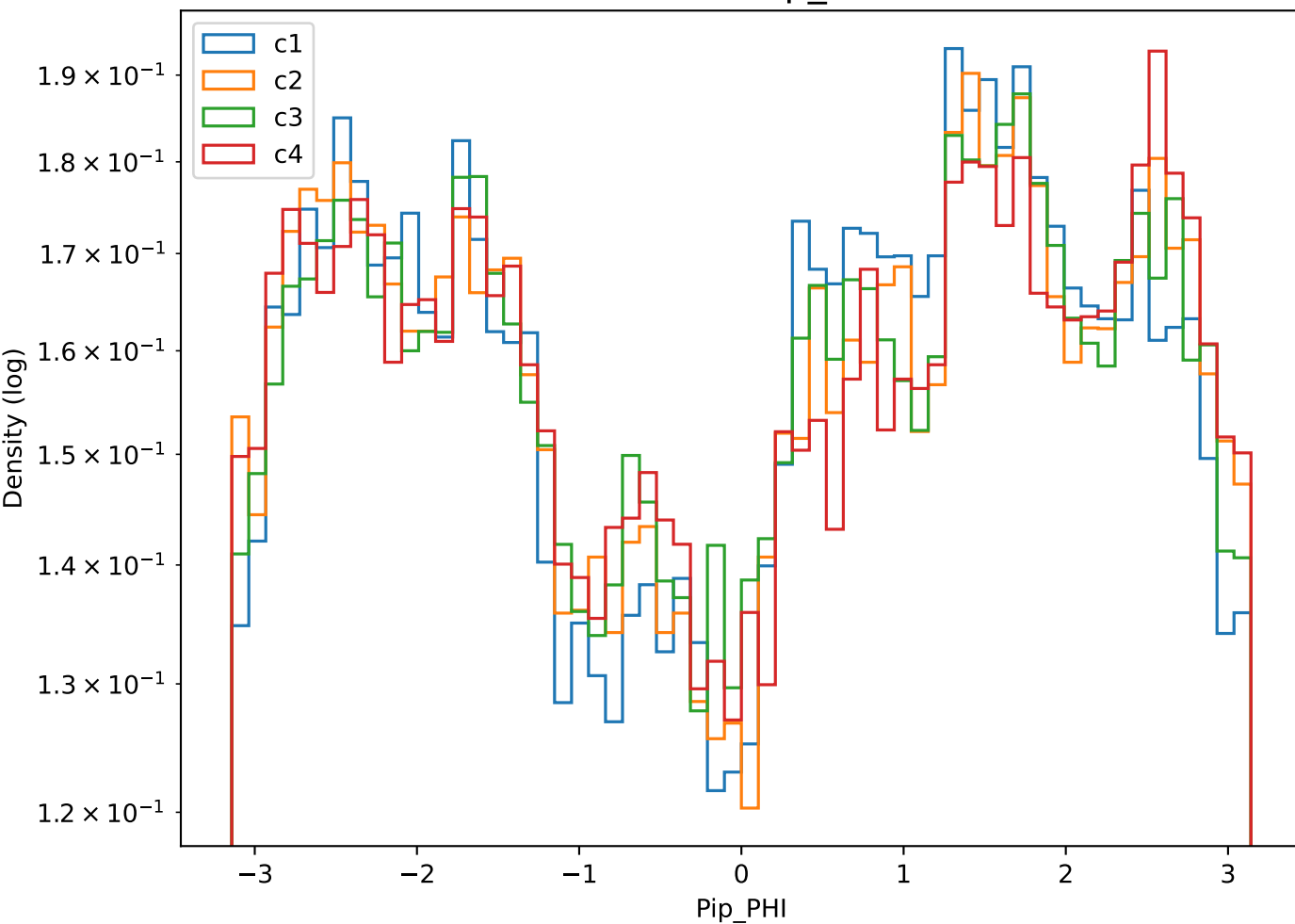
Branch: Pip_PHI
