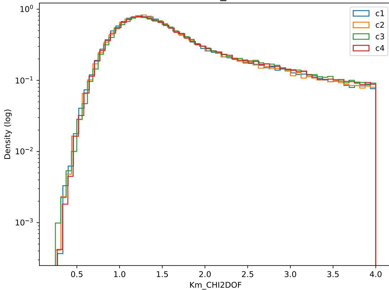
Branch: Km_CHI2DOF
