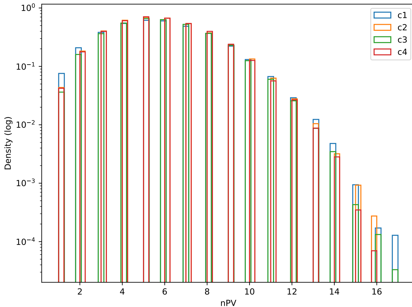
Branch: nPV
