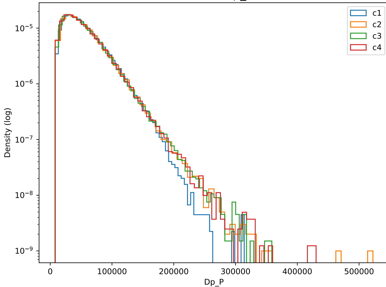
Branch: Dp_P
