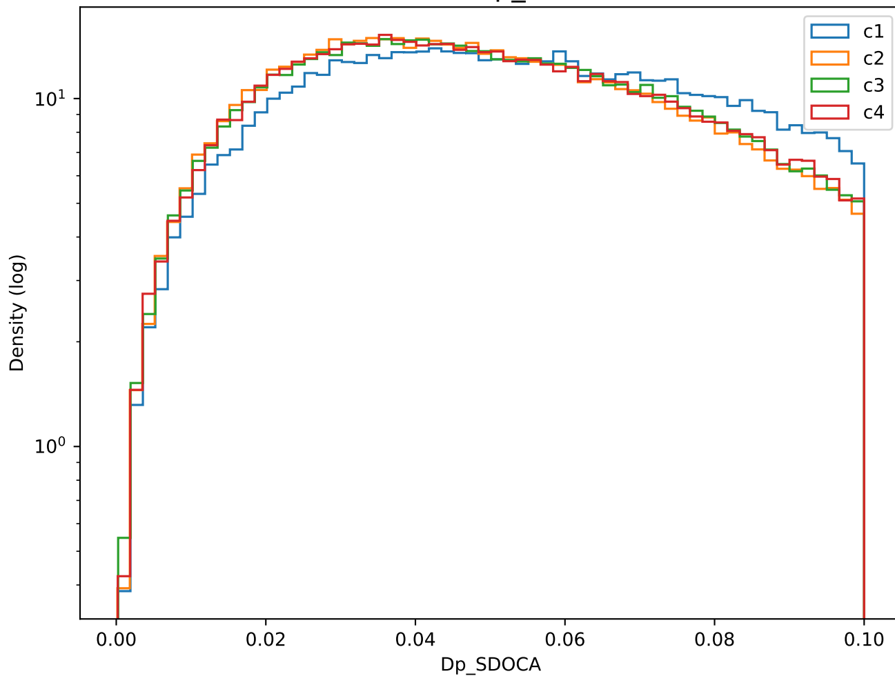
Branch: Dp_SDOCA
