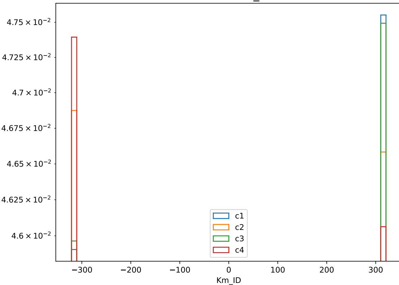
Branch: Km_ID
