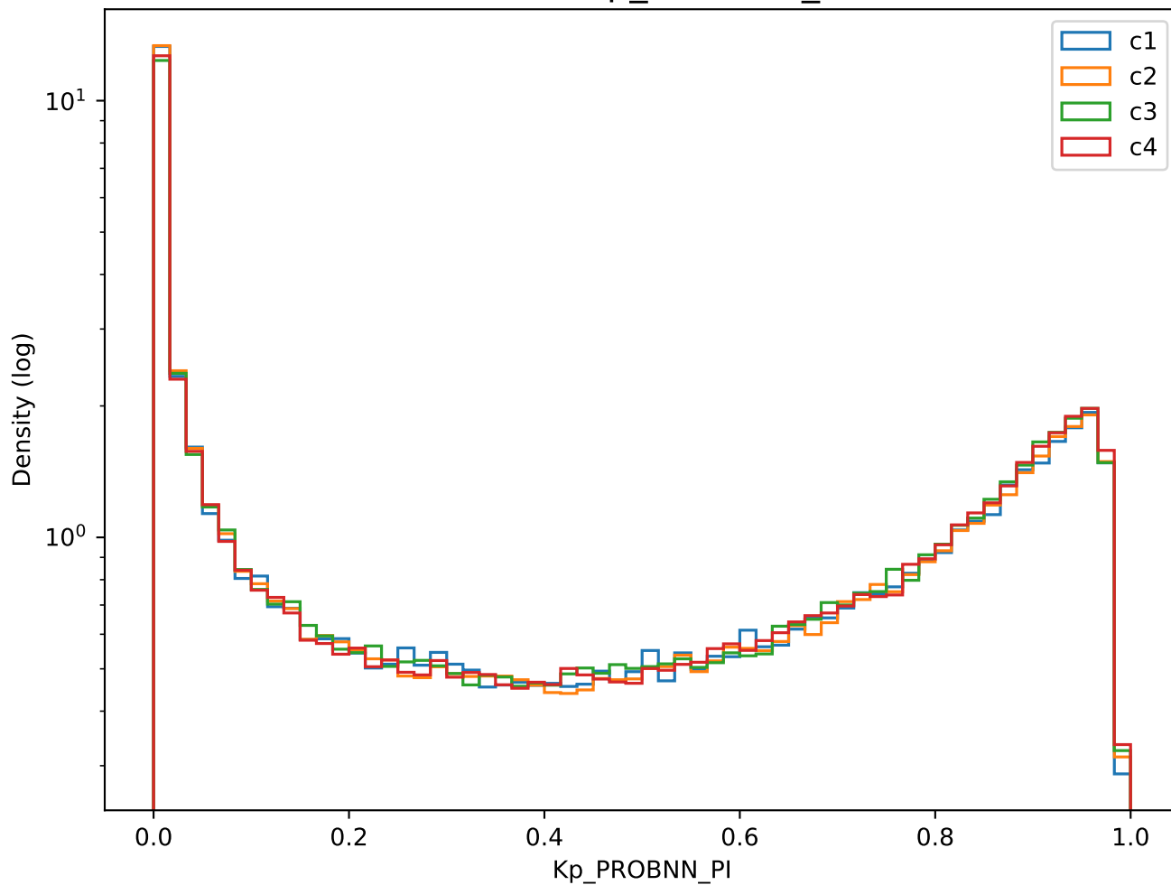
Branch: Kp_PROBNN_PI
