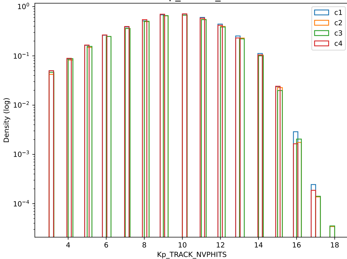
Branch: Kp_TRACK_NVPHITS
