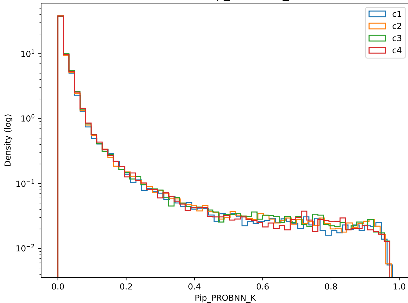
Branch: Pip_PROBNN_K
