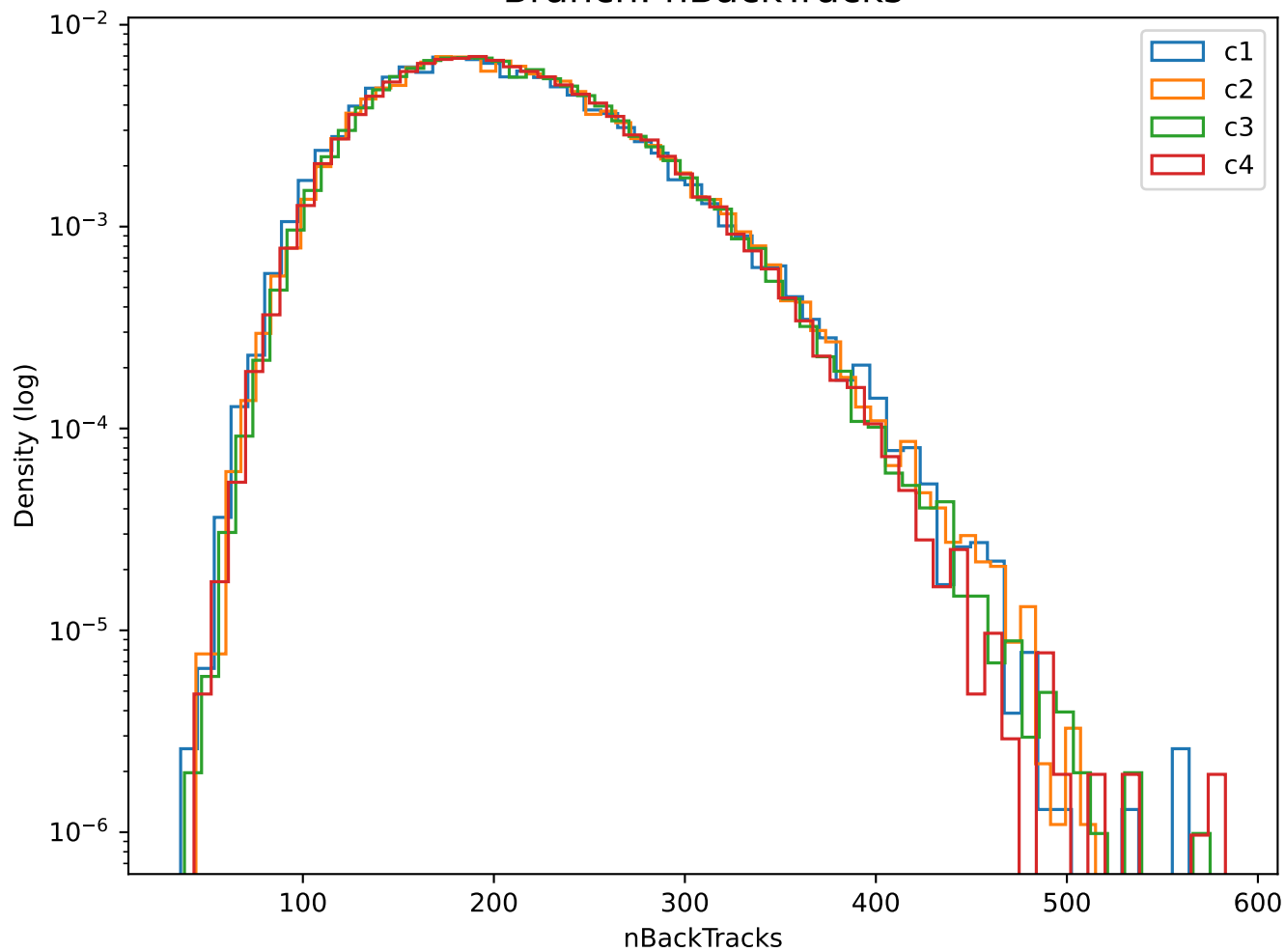
Branch: nBackTracks
