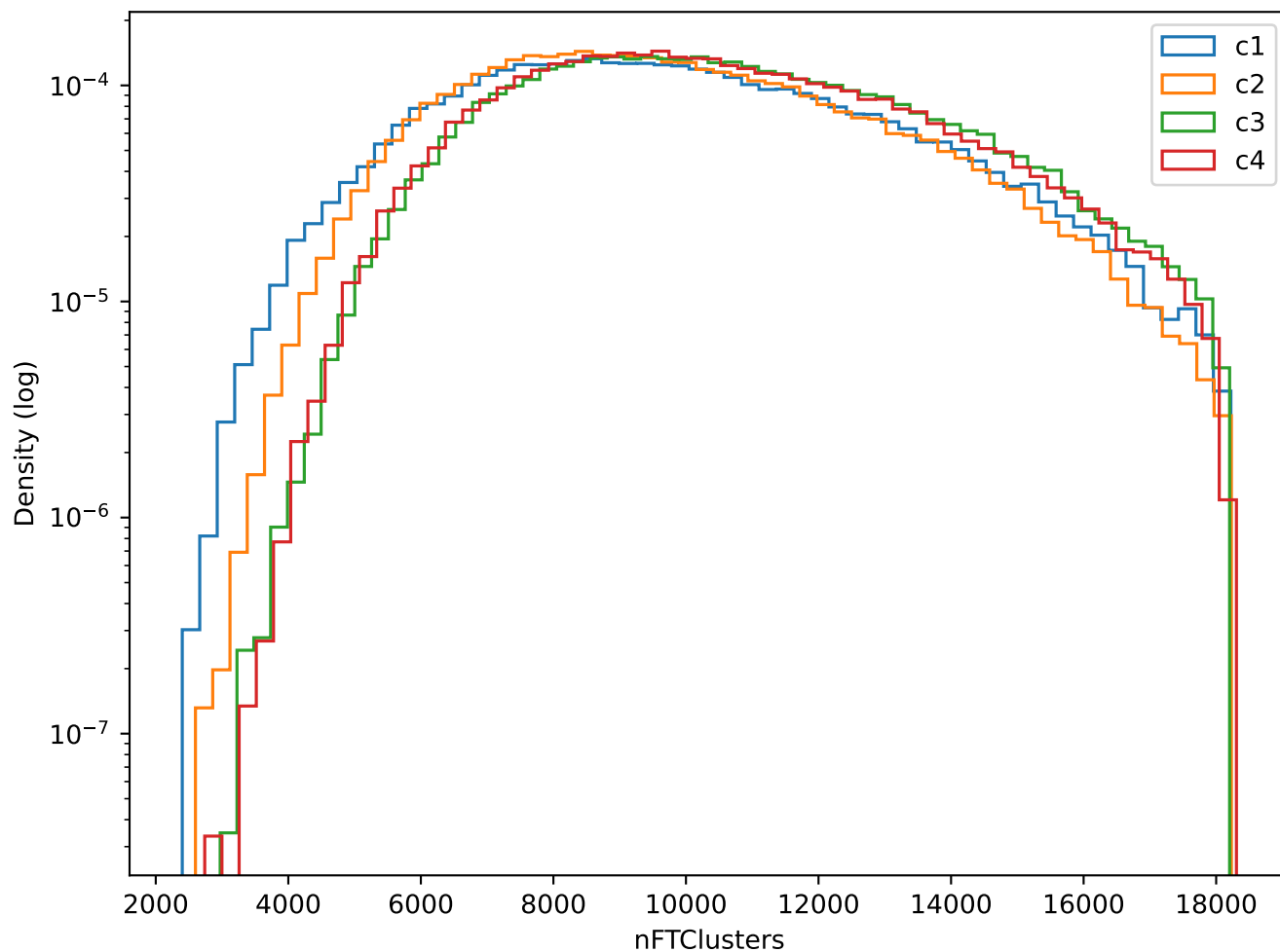
Branch: nFTClusters
