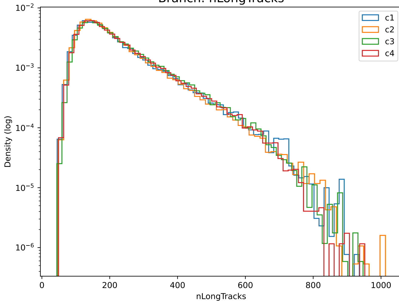
Branch: nLongTracks
