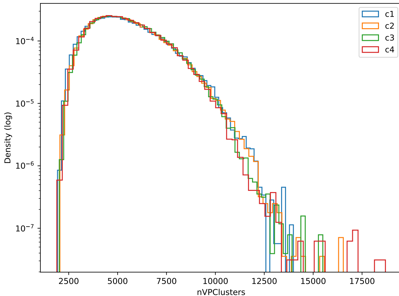
Branch: nVPClusters
