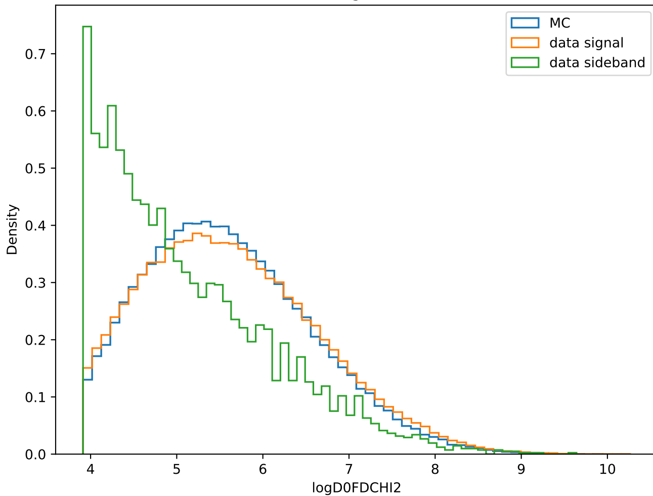
Branch: logD0FDCHI2
