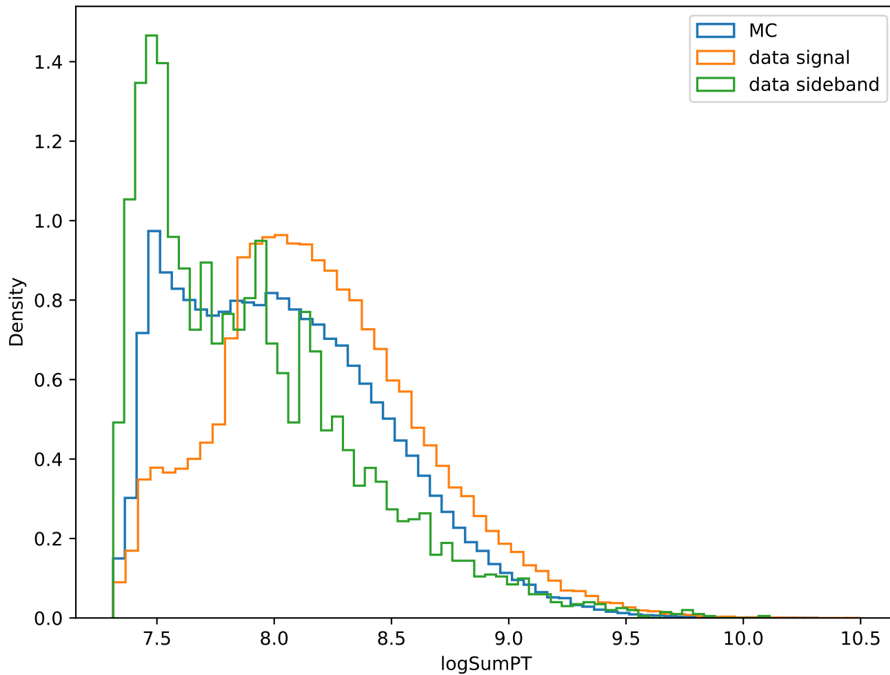
Branch: logSumPT
