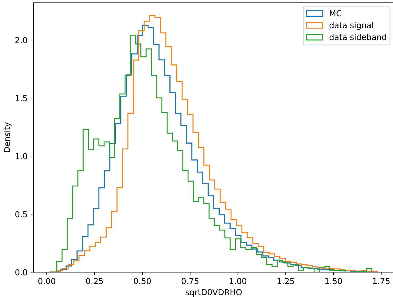
Branch: sqrtD0VDRHO
