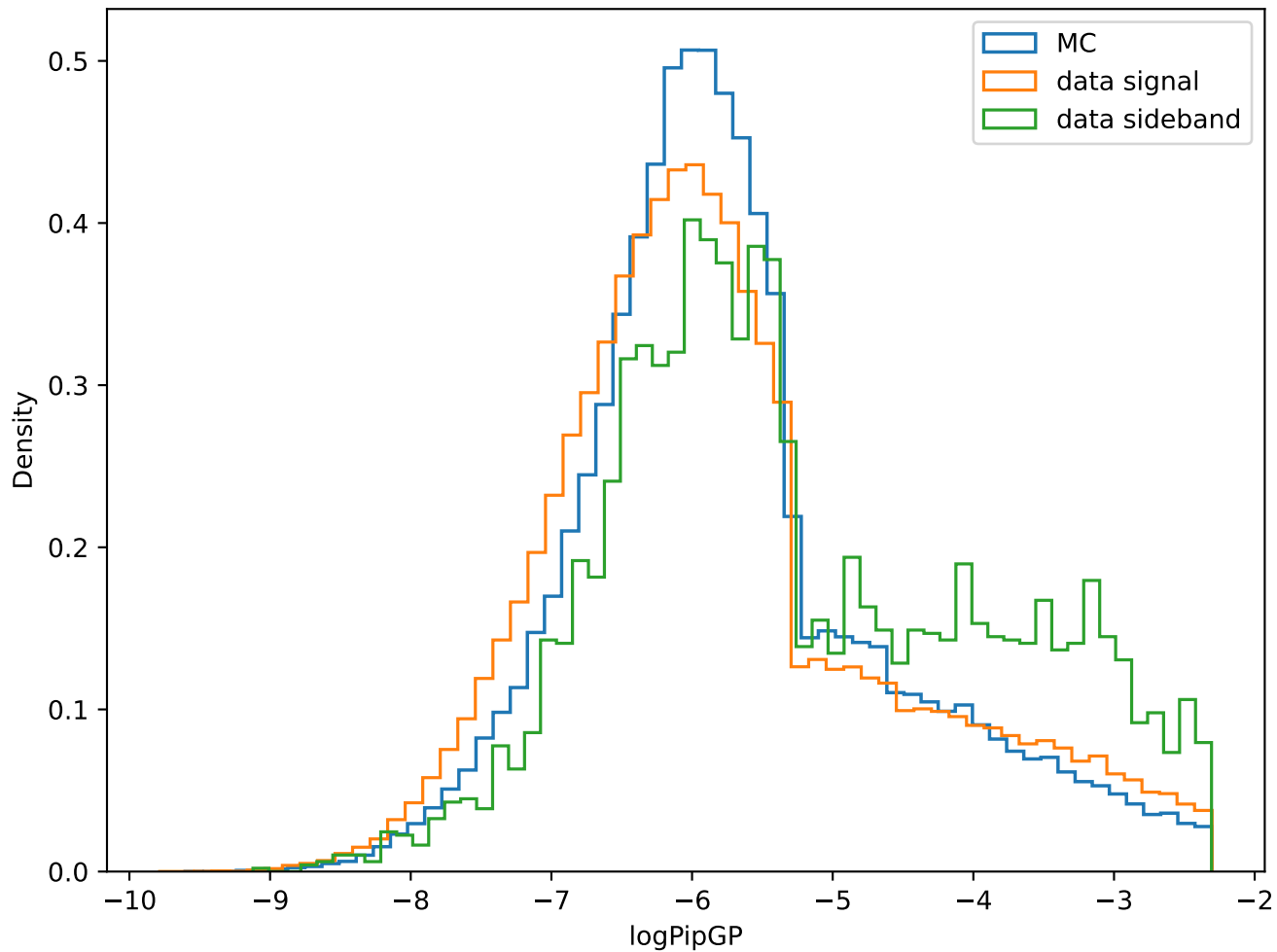
Branch: logPipGP
