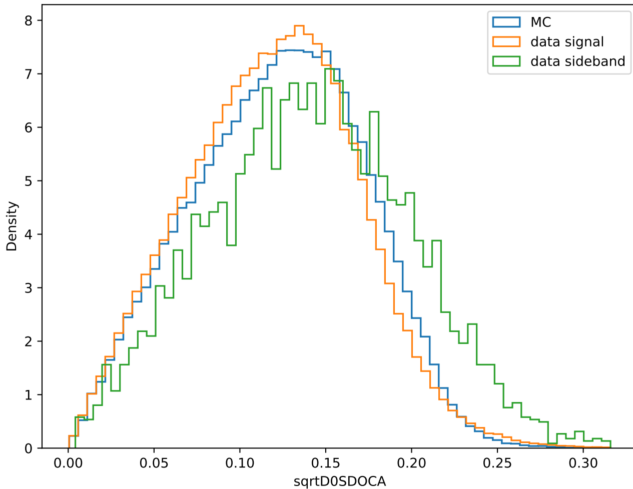
Branch: sqrtD0SDOCA
