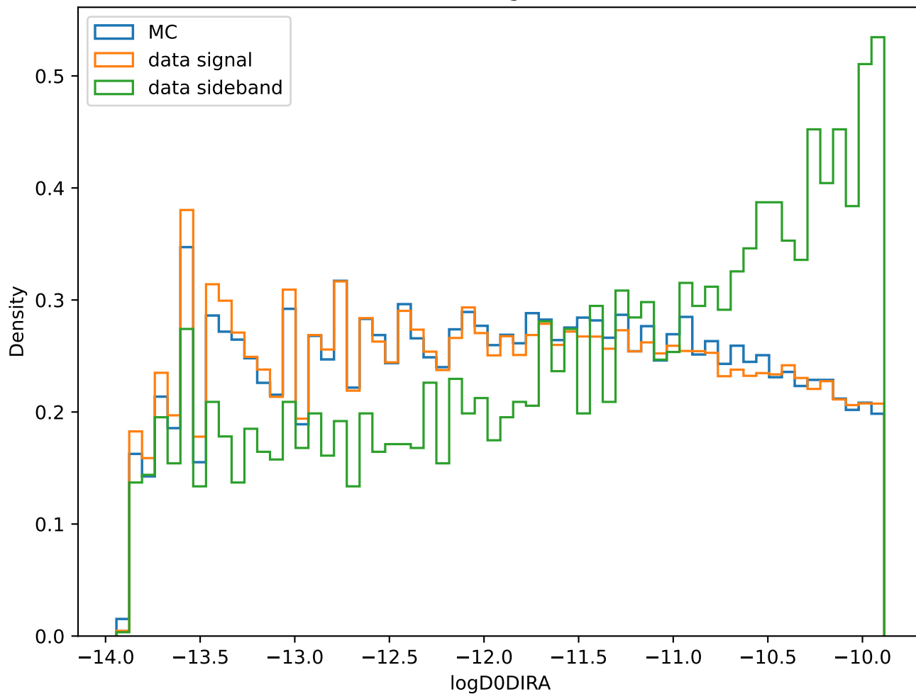
Branch: logD0DIRA
