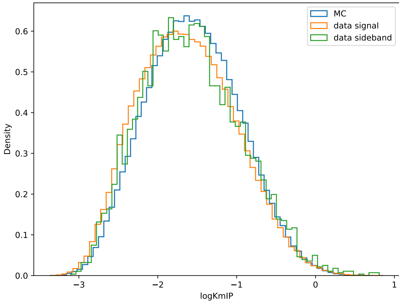
Branch: logKmIP
